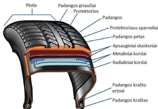
1 pav. Padangos sudedamosios dalys ( www.azom.com/article.aspx... )
