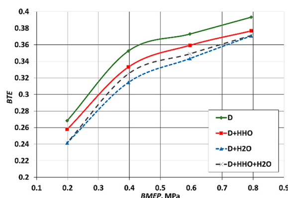
Figure 5. The BTE vs. BMEP with various fuel mixtures (and water injection).
