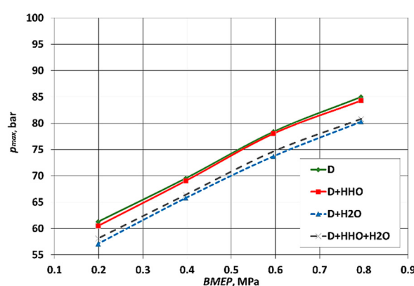
Figure 3. In-cylinder maximum pressure vs. BMEP with various fuel mixtures (and water injection).
