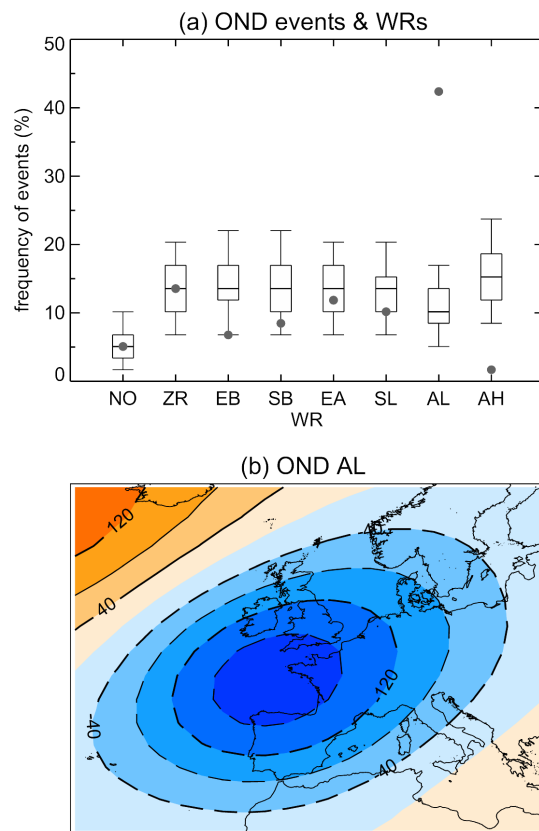
Figure 8. (a) Relative frequency of autumn extreme daily mean de-trended water heights above the 99.5th percentile of the 1948–2018 (in per cent with respect to the total number of events) occurring under the given weather regime (WR). Whiskers denote the random distributions obtained from a bootstrap of 5000 trials, each one containing the same number of autumn days of the 1948–2018 period as surge events. Boxes denote the inter-quartile distribution, with the median in between, and bars extend from the 5th to the 95th percentile of the random distributions. WRs are defined from daily fields of geopotential height at 500 hPa of the NCEP/NCAR reanalysis over the Euro-Atlantic sector [30, 65]° N, [30° W, 25° E]. Abbreviations are as follows: NO – no (i.e. undefined) WR, ZR – zonal regime, EB – European blocking, SB – Scandinavian blocking, EA – East Atlantic, SL – Scandinavian low, AL – Atlantic low, AH – Atlantic high. See Garrido-Pérez et al. (2020) for further details. (b) The AL pattern that is associated with the occurrence of more than 40 % of extremes. Data sources: NCEP/NCAR reanalysis (Kalnay et al., 1996).
