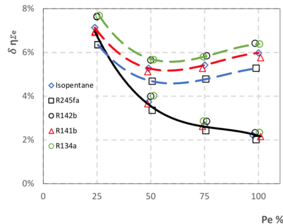
Figure 5. ORC realization strategy to influence the increase in ship power plant COP \eta_{\Sigma e} ; G_{w.fl.} = const (—); G_{w.fl.} = var. (—); blue line: Dry fluid; red line: Isentropic/Dry fluids; and green line: Wet/Isentropic fluids.
