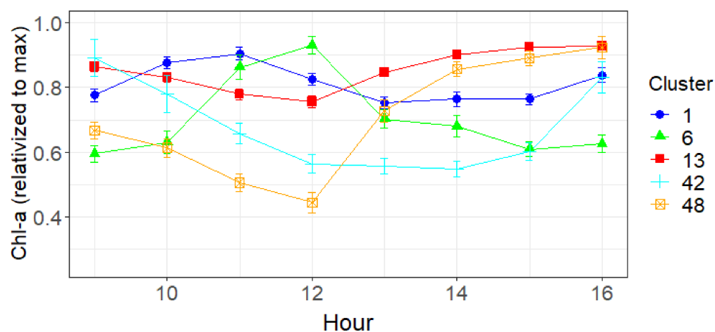
Figure 5. Average hourly (UTC time) Chl-a (with standard error), relativized to maximum value per day.
