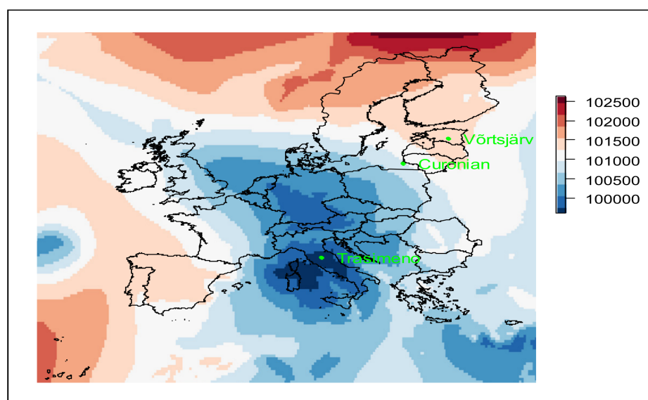
Figure 1. Map of Europe showing the three WISPstation sites together with atmospheric pressure (Pa) on the 28 July 2019 indicating the weather system that marked the end of the July heatwave.
