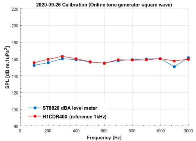
Figure 3. The frequency response to a square wave signal at different frequency bands of the recording setup
