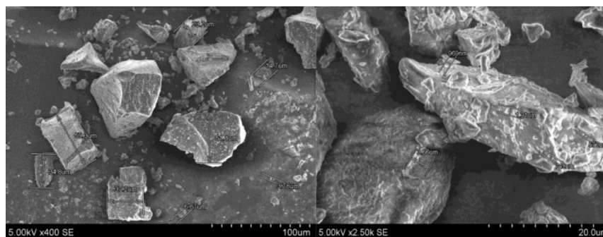
Figure 2. Ball milled mucilage binder particles image obtained employing Hitachi S-3400N SEM with a 5.00 kV energy.
