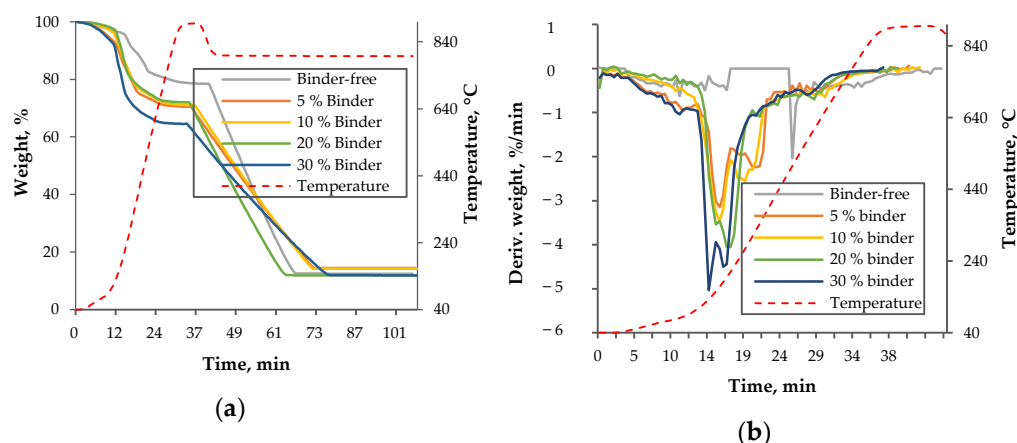
Figure 5. Thermal analysis of activated algal biochar mixed with different concentrations of the mucilage binder: (a)—TG curve; (b)—DTG curve obtained before combustion initiation.
