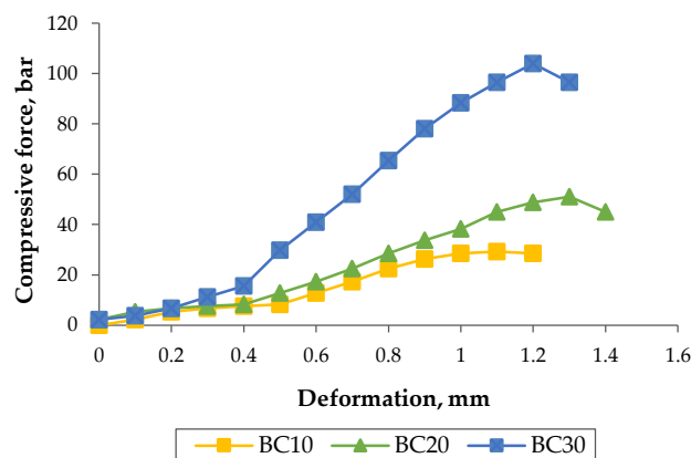
Figure 6. Compression deformation experiment results of biochar anodes with different binder concentrations.
