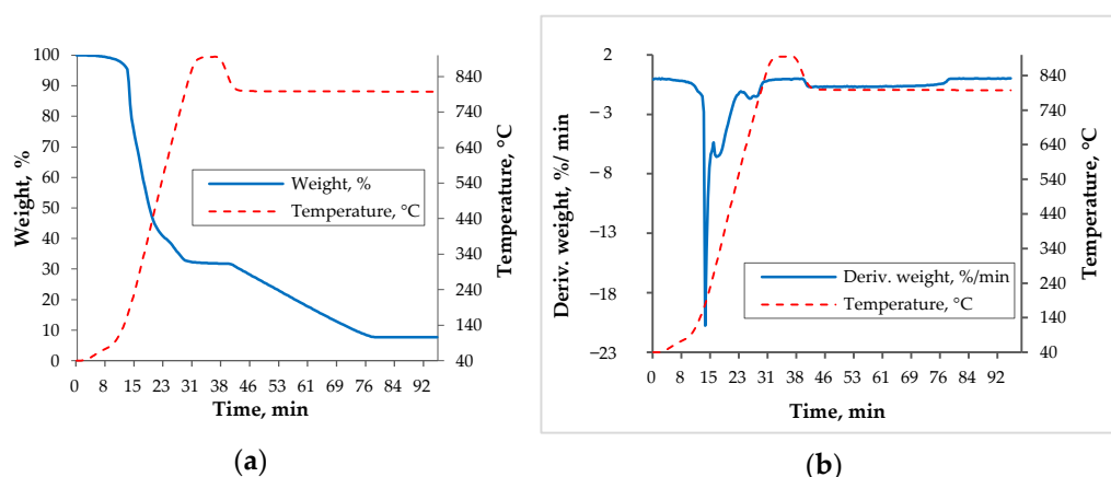
Figure 4. Thermal analysis of red seaweed (Rhodophyta) feedstock: (a) thermogravimetric (TG) curve; (b) derivative thermogravimetric (DTG) curve.
