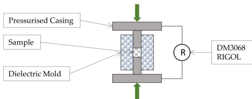
Figure 3. The system of two-part compression mold.
