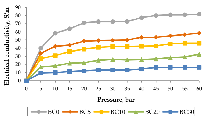
Figure 9. Dependence of calculated electrical conductivity values on the pressure applied to samples with different concentrations of the binder.
