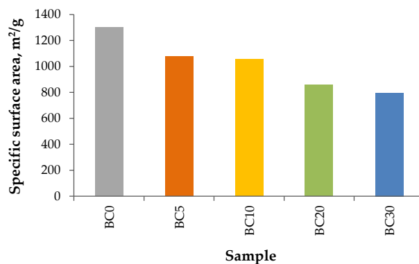
Figure 7. Dependency of binder concentration (wt.%) on the specific surface area of formed anode.
