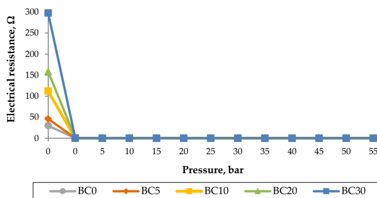
Figure 8. Experimentally measured electrical resistance value ( \Omega ) dependency on the pressure applied to the surface of anode sample.
