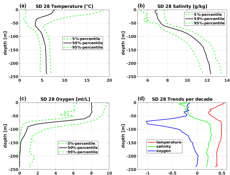
Figure 2. Observed temperature (a), salinity (b), and oxygen (c) data as a function of depth and time. Subdivision 28 (SD 28, eastern Gotland Basin) for the period 1979–2018. Data from the ICES Marine Data Centre ( https://www.ices.dk/Pages/default.aspx , last access: 12 August 2019).
