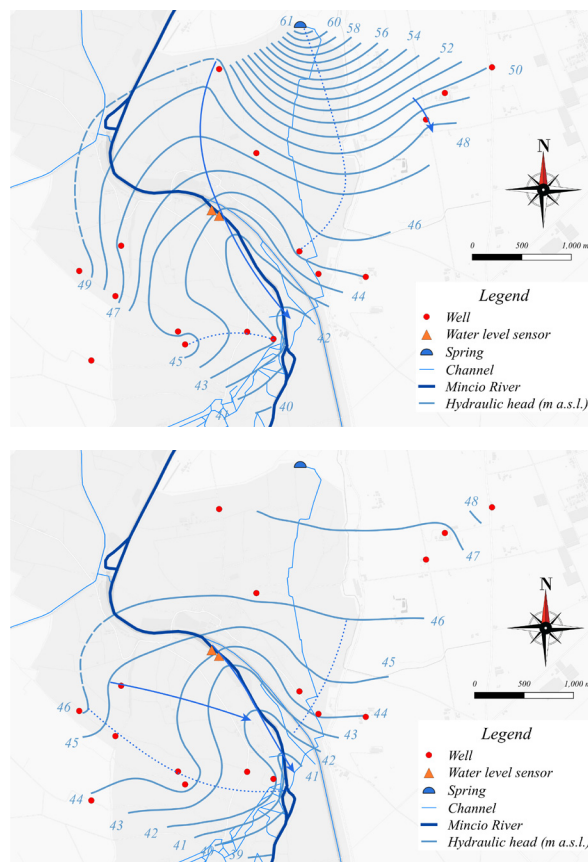
Fig. 5 - top) Net groundwater flow in July 2019, during the irrigation period; bottom) Net groundwater flow in December 2019. The dotted blue lines represent groundwater divides and the blue arrows drainage axes
