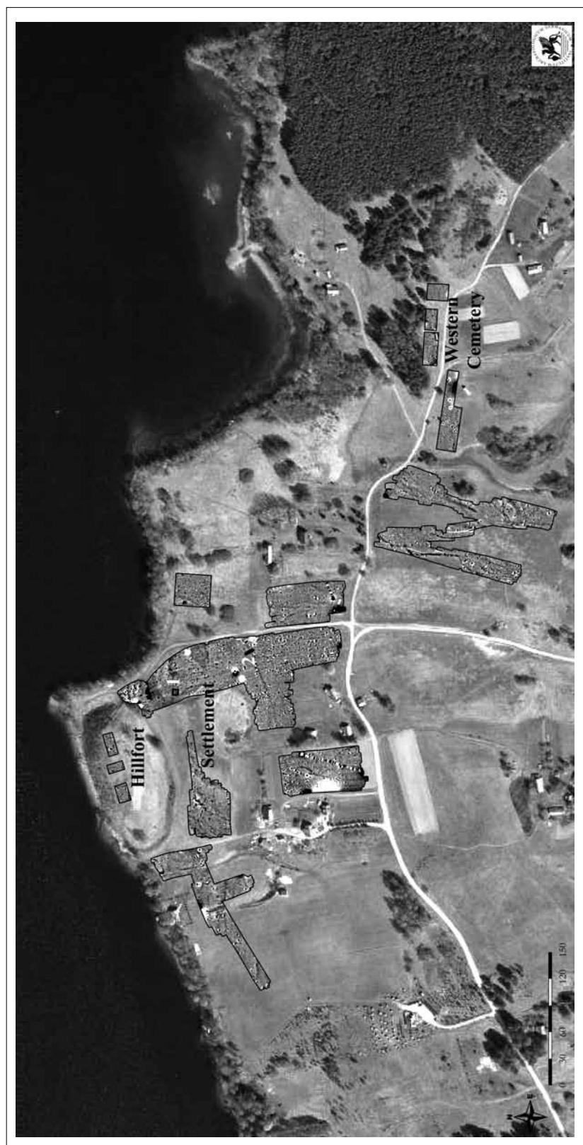
Fig. 12. Taurapilis. Geomagnetic surveys 2011-2012, areas of investigation ( -20/+20 nT); 1-2 archaeological trenches 2012.
