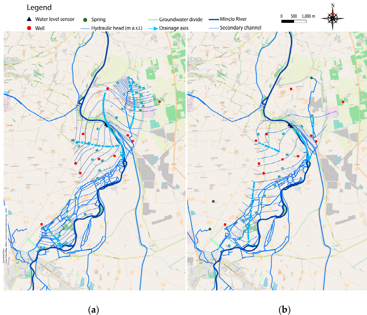
Figure 2. Potentiometric maps. (a) Potentiometric map of August 2020; (b) Potentiometric map of March 2021. Basemap from OpenStreetMap ( https://www.openstreetmap.org , accessed on 6 December 2021).
