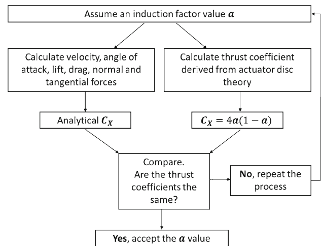
Fig. 16 Block diagram of DMST working mode
