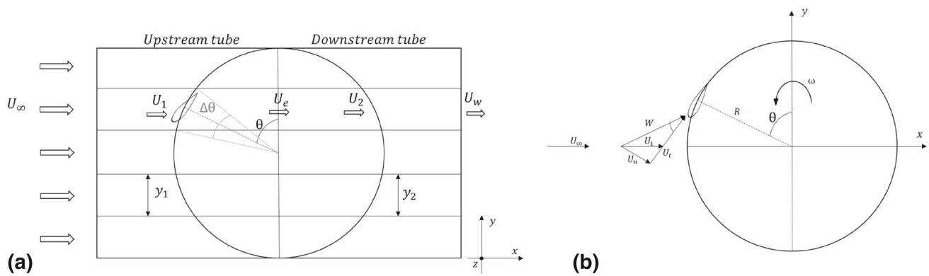
Fig. 17 a Generical horizontal plane of the turbine for DMST reference; b schematic representation of velocity involved in DMST calculations
