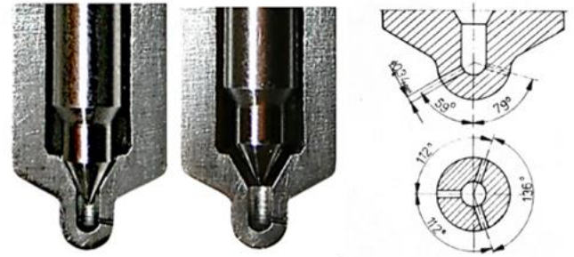
Fig. 1. Geometric parameters of D1LMK 148/1 atomizer used at the test stand
