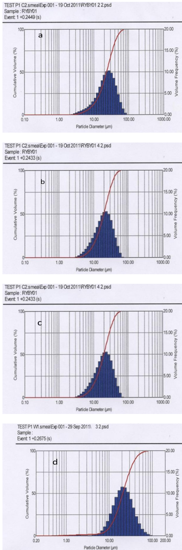
Fig. 9. Distribution of drops of the injected reference fuel: a, b, c and d – fuel injection start pressure, respectively 20.0; 22.0; 24.0 and 26.0 MPa
