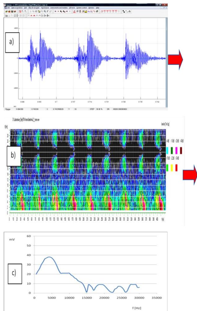
Fig. 7. Recorded source signal (a), transformation of source signal into time-frequency spectrogram and determination of the frequency band with the maximum signal (b), determination of acoustic emission signal energy in recorded frequency band at a specific moment in time (c)
