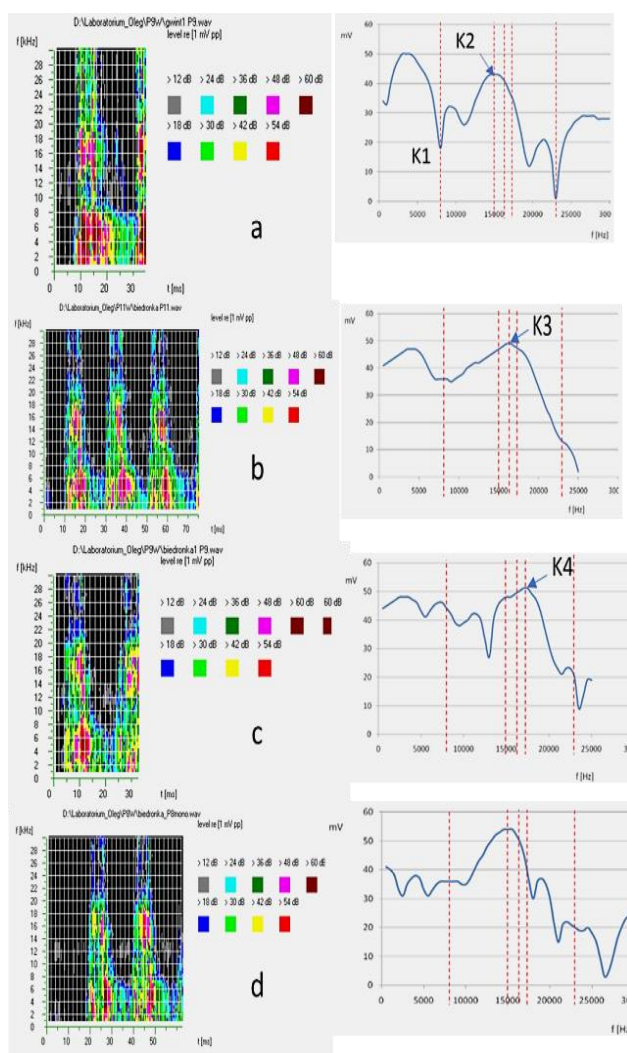
Fig. 8. Time-frequency spectrograms and energy of the EA signal in the recorded frequency band at a specific moment in time for the reference fuel: a, b, c and d – fuel injection start pressure, respectively 20.0; 22.0; 24.0 and 26.0 MPa; K1, K2, K3, K4 – reference points
