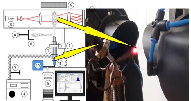
Fig. 5. Scheme of the experimental device for determining the quality of the atomized fuel and acoustic emission: 1 – nozzle, 2 – nozzle attachment point, 3 – Spraytec STP 5000 device, 4 – EPS 200 installation, 5 – personal computer, 6 – spray catchers, 7 – fume hood, 8, 9 – thermocouples, 10 – acoustic emission sensor, 11 – acoustic tester
