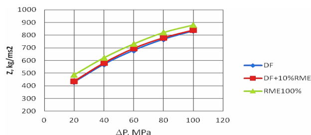
Fig. 3. Acoustic resistance change ( Z ) as a function of the pressure of selected fuels injection
