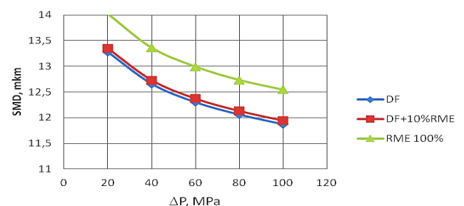
Fig. 2. Change of the average diameter of atomized fuel drop depending on the injected fuel pressure
