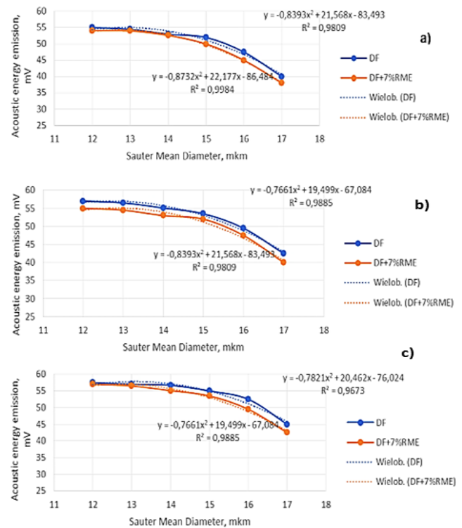
Fig. 10. Relationship between Sauter mean diameter of atomized fuel drop and level of the acoustic emission formed in the atomization process for the start fuel injection pressure: a – 22.0 MPa; b – 24.0 MPa; c – 26.0 MPa
