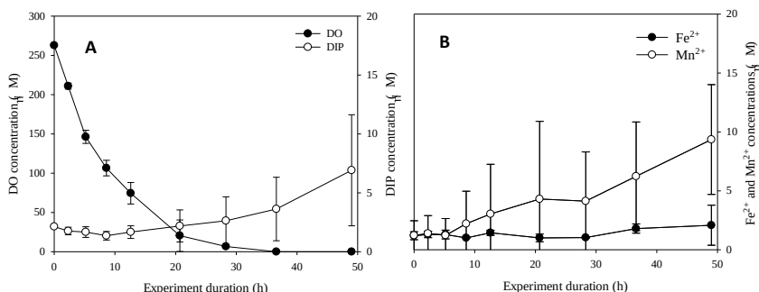
Fig. 4.12 Dynamics of dissolved oxygen (DO) and inorganic phosphorus (DIP, A), iron and manganese (B) concentrations in near-bottom water during oxic and anoxic incubations of sediment cores from Curonian lagoon (average \pm SD, n = 4 )
