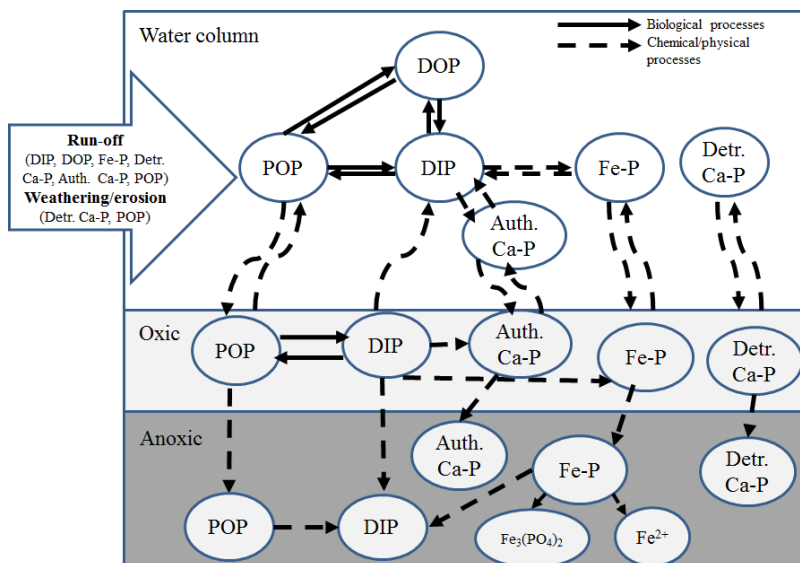
Fig. 1.2 Phosphorus cycle in the water column and sediment (modified from Reddy et al., 2005)
