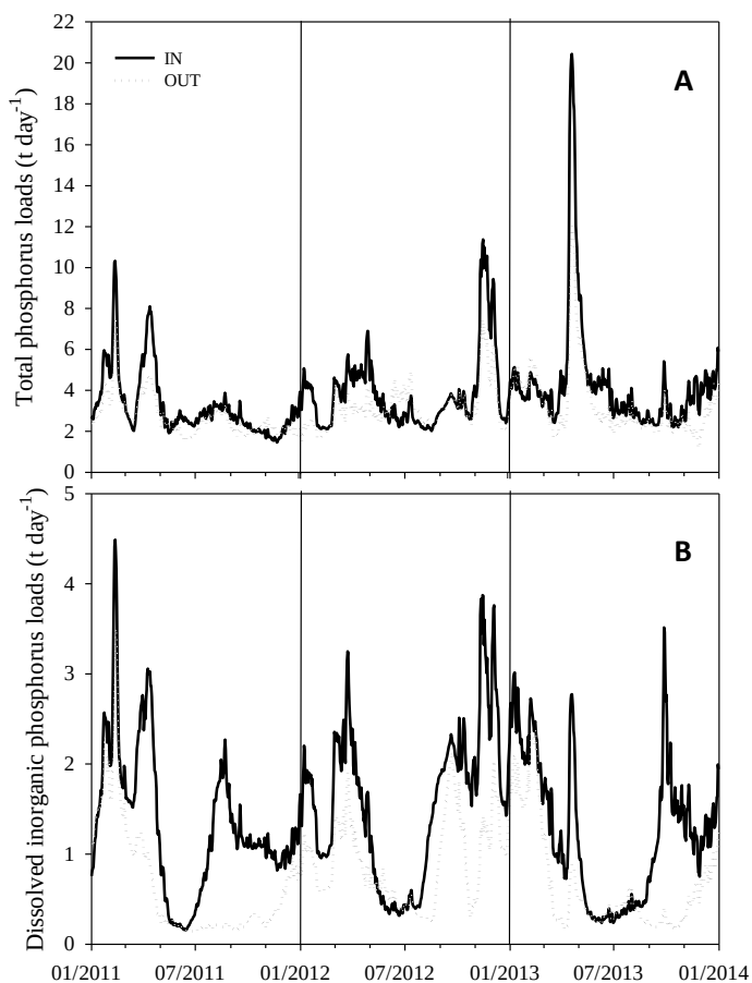
Fig. 4.16 Total (TP; A) and dissolved inorganic (DIP; B) phosphorus loads inflowing to (IN) and outflowing from (OUT) the Curonian lagoon in 2011–2013. Note different Y scales.
