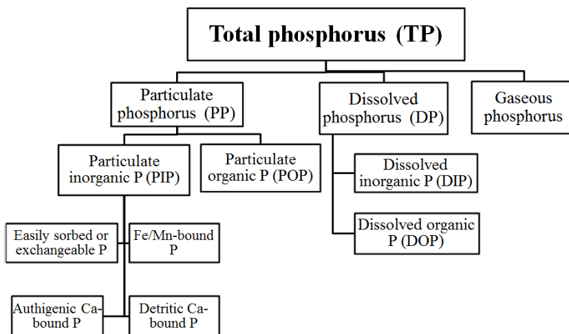
Fig. 1.1 Basic phosphorus forms in water column and sediments
