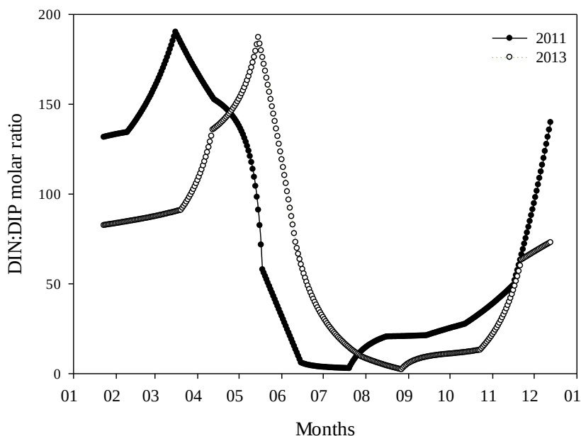
Fig. 4.18 Molar ratios of dissolved inorganic nitrogen (DIN) and phosphorus (DIP) calculated in the Nemunas River water at the closing section in 2011 (black circle) and 2013 (open circle)
