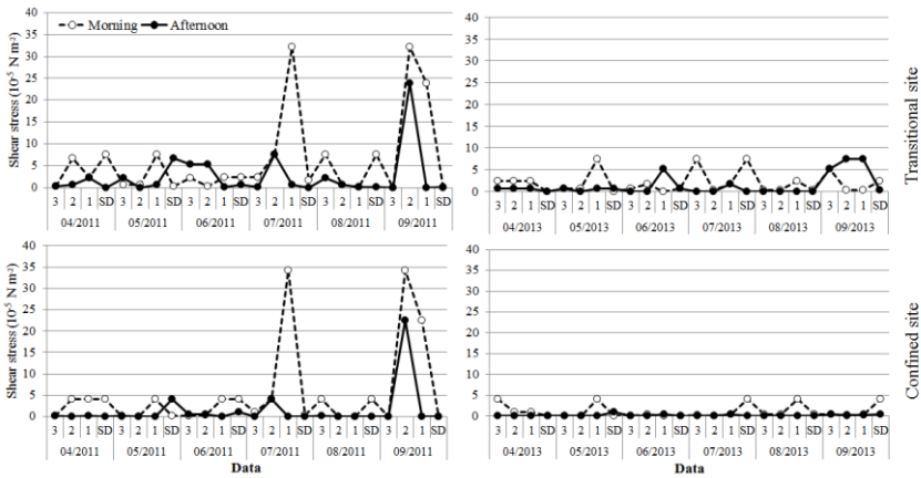
Fig. 4.3 Wind induced shear stress at transitional and confined sites in 2011 and 2013 (SD – sampling days; numbers (1, 2, 3) of days before sampling at morning (6 am) and afternoon (6 pm))
