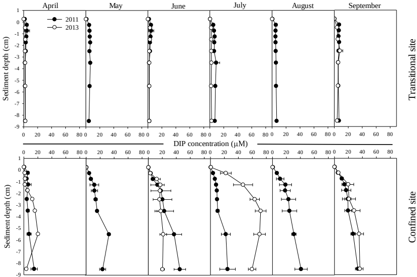
Fig. 4.10 Dissolved inorganic phosphorus (DIP) concentration in porewater of sediments in the Curonian lagoon (average \pm SD, n=3 )
