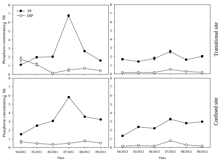
Fig. 4.4 Total (TP) and dissolved inorganic (DIP) phosphorus concentration in water column (2011 TP concentrations were provided by Marine Research Department, data interpolation was
