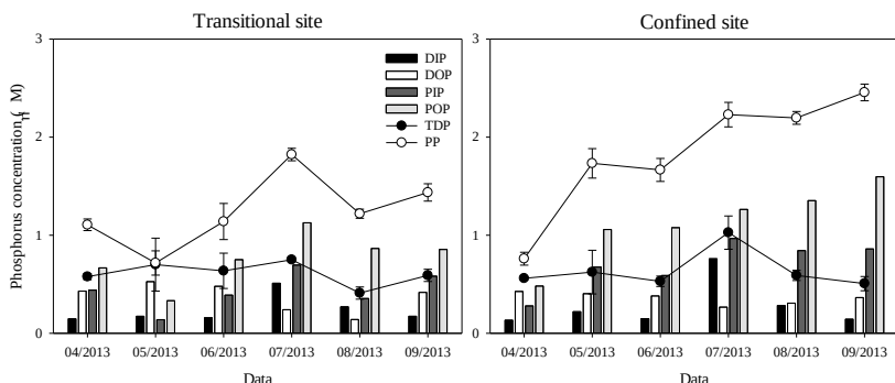
Fig. 4.5 Seasonal concentrations of phosphorus forms (DIP – dissolved inorganic phosphorus, DOP – dissolved organic phosphorus, PIP – particulate inorganic phosphorus, POP – particulate organic phosphorus, TDP – total dissolved phosphorus, PP – total particulate phosphorus) in water column of the Curonian lagoon (average \pm SD; n=3 )
