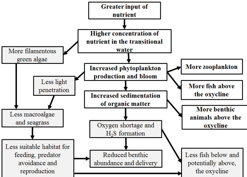
Fig. 1.4 Schematic representation of cascading effects of the eutrophication process. Grey box represents the harmful effect. (modified from Rönnerberg and Bonsdorff 2004 and Rabalais et al. 2009)
