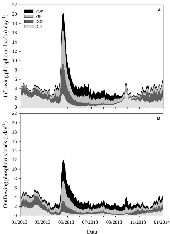
Fig. 4.17 Speciation of phosphorus (P) forms in inflowing (A) and outflowing (B) loads in 2013. POP – particulate organic P, PIP – particulate inorganic P, DOP – dissolved organic P and DIP – dissolved inorganic P
