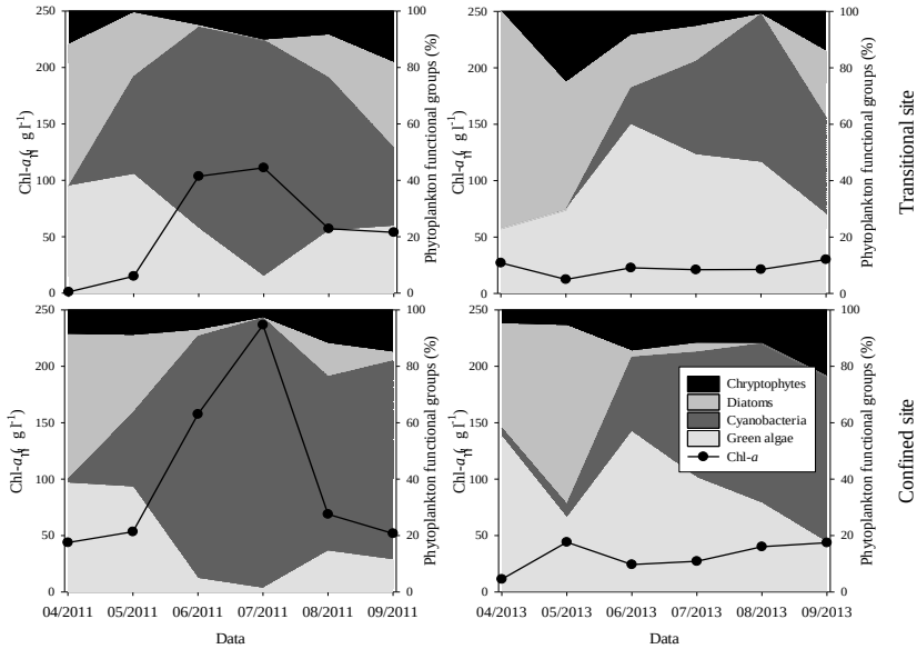
Fig. 4.1 Chl-a and phytoplankton functional groups during study years at transitional and confined sites
