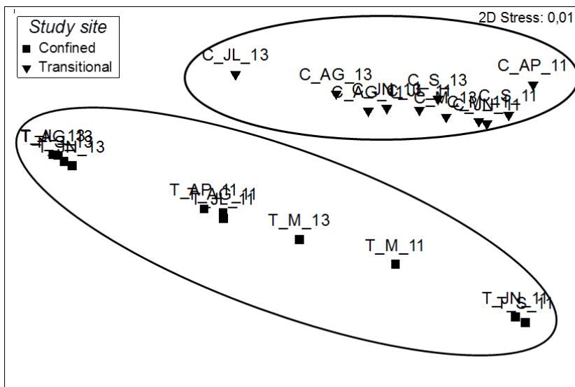
Fig. 4.11 Multidimensional scaling (MDS) analysis of sedimentary characteristics. Data labels corresponding study sites (T – transitional, C – confined), sapling months (AP – April, M – May, JN – June, JL – July, AG – August, S – September) and years (11 – 2011, 13 – 2013).
