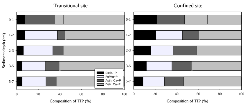
Fig. 4.9 Inorganic phosphorus forms (TIP) in transitional and confined sites with sediment depth in 2013 (the average of June and September values)
