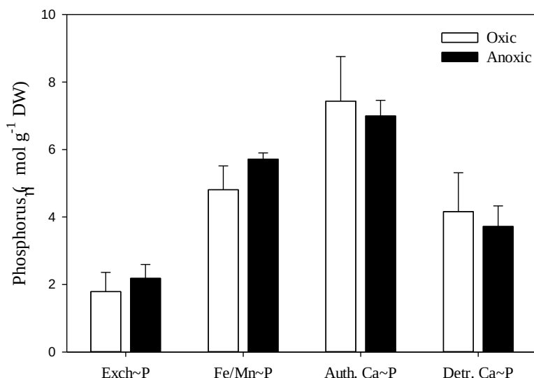
Fig. 4.15 Sedimentary inorganic phosphorus pools before and after anoxia creation in the surface of sediments (average \pm SD, n=3 )
