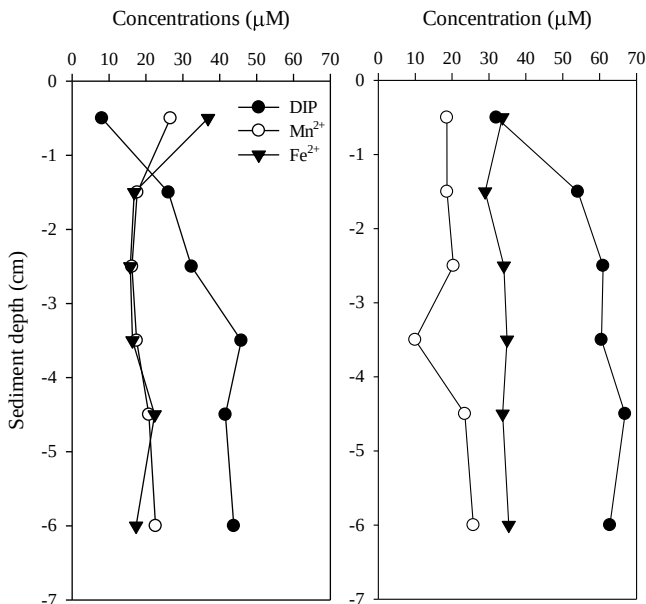
Fig. 4.14 Porewater profiles of DIP, Mn^{2+} and Fe^{2+} in oxic and anoxic conditions in confined site sediment (average \pm SD, n=3 )
