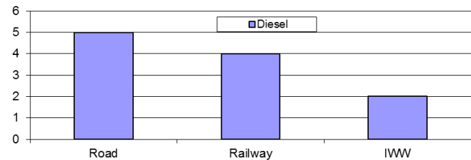
Figure 13. Generated SO 2 emission in kilograms for the transportation of 80 TEU using diesel fuel (using LNG fuel SO 2 emission close to 0) by different transport roads.
