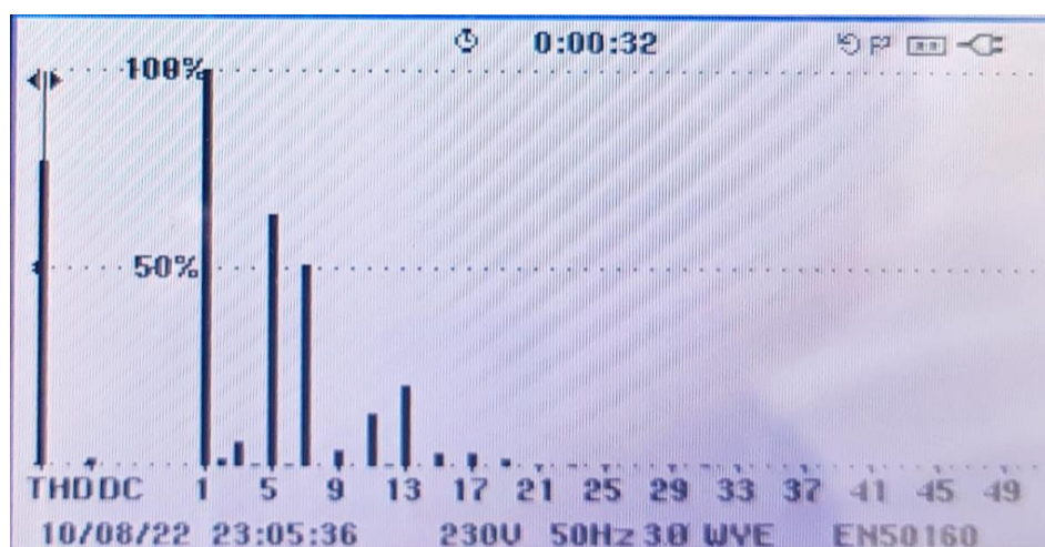
Figure 6: Current spectrum.
