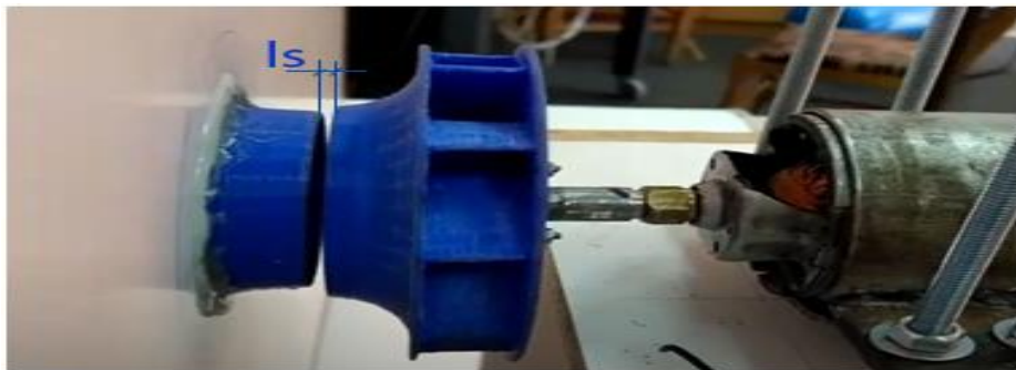
Figure 5: The fan in the test device. Gap Is .
