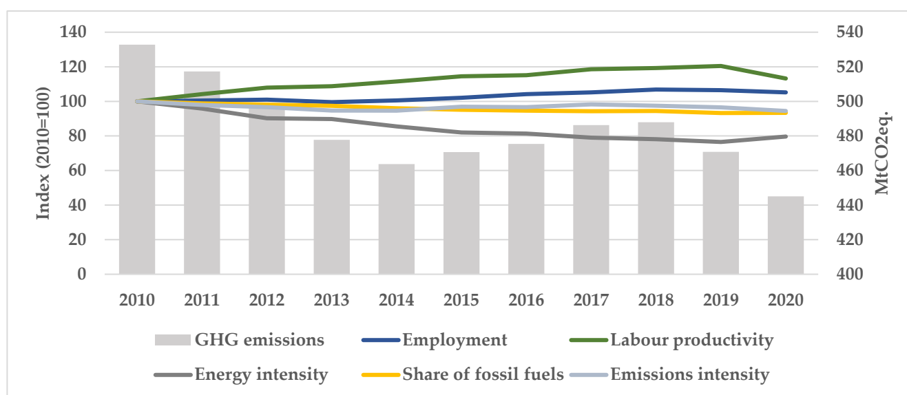
Figure 6. Changes in associated GHG emissions and their key drivers in the EU–27 (own estimations based on [55–58]).
