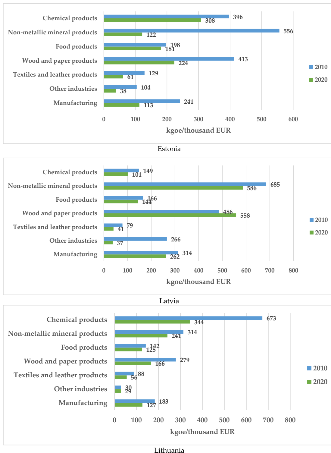
Figure 2. Energy intensity in manufacturing branches of the Baltic States in 2010 and 2020 (own estimations based on [49–54]).
