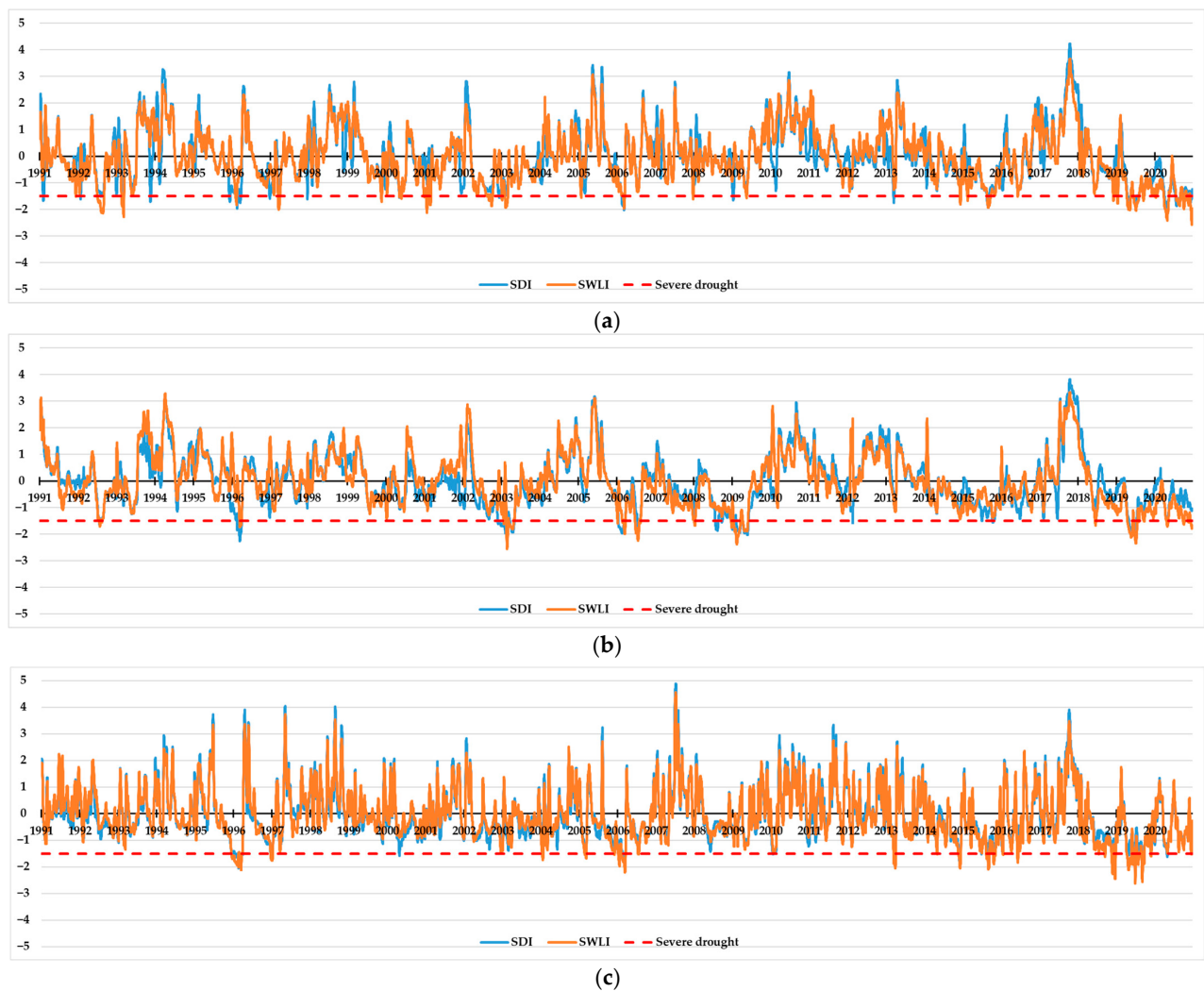
Figure 4. Comparison between SWLI and SDI over 30 years: (a) Nemunas-Smalininkai; (b) Žeimena-Pabradė; (c) Šešuvys-Skircgailai.
