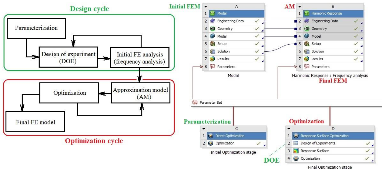
Fig. 3. Flowchart of the optimization task in ANSYS software.
