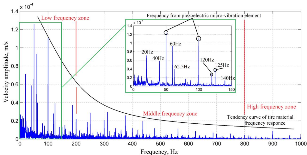
Fig. 6. The frequency response of composite tire surface from measurements.
