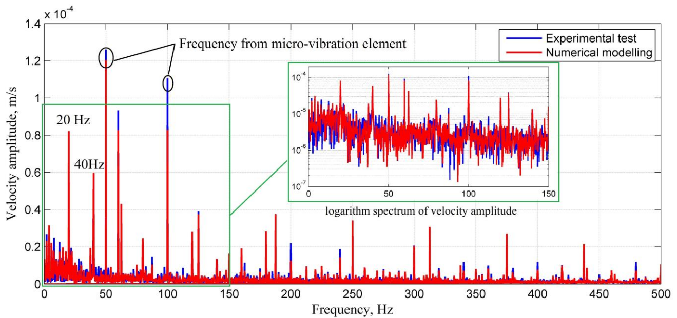
Fig. 7. Comparison of frequency responses between experimental and numerical research: a) spectrum of deformation amplitude; b) spectrum of velocity amplitude.
