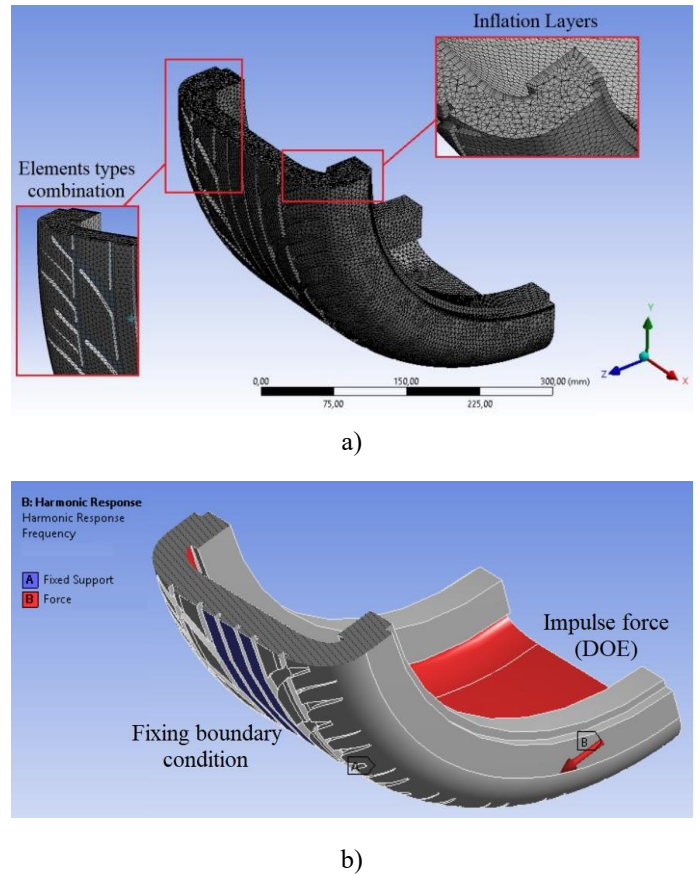
Fig. 2. View of numerical model parameters: a) example of grids in mesh independence study; b) view of the boundary conditions for numerical modelling.
