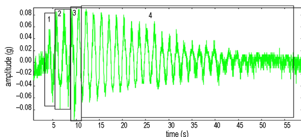
Fig. 9. Manually operated crane with empty container accelerations
