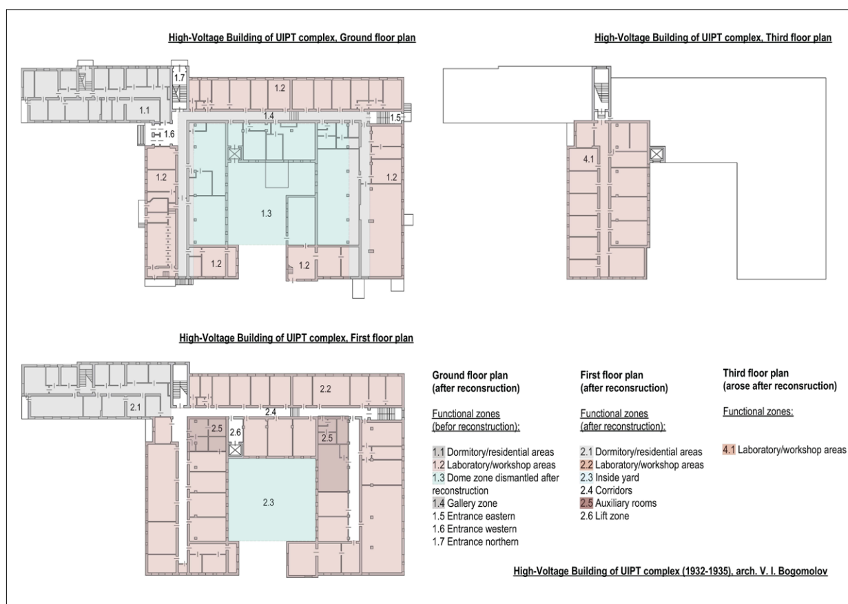
Fig. 8. High-Voltage Building, plans; by K. Didenko and O. Bondarchuk, from the archives of the NSC KhIPT
