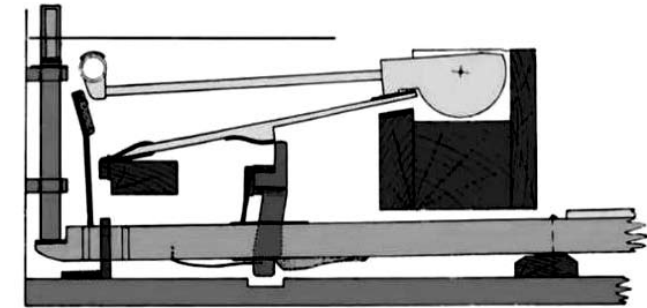
Piano Action of B. Cristofori piano
