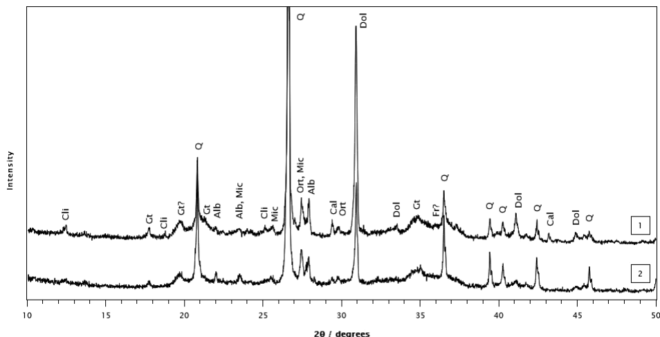
Fig. 10. XRD patterns of ore samples. Explanations: Alb – albite; Cal – calcite; Cli – Clinocllore; Dol – dolomite; Fr – ferrihydrite; Gt – goethite; Mic – microcline; Ort – orthoclase; Q – quartz.
