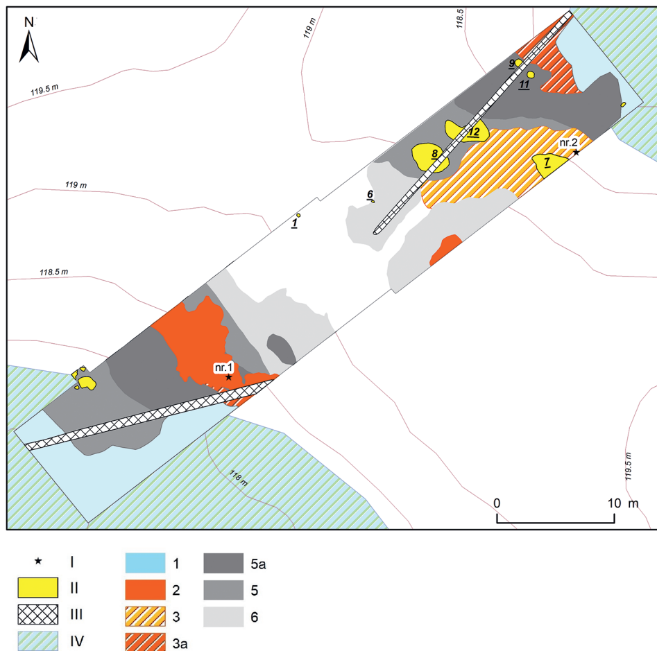
Fig. 4. Excavated area of the Mikniškiai settlement: I – locations of iron ore samples; II – sunken features (only anthropogenic features are numbered); III – drainage; IV – peaty wetlands. Areas of layers and horizons: 1 – greyish clay; 2 – cemented limonite; 3 – limonized clay loam; 3a – grey sandy loam with randomly spread iron ore concretions or limonized soil; 5a – blackish loamy soil with charcoal; 5 – grey loamy soil mostly with charcoal; 6 – a plough-affected grey loamy soil with sparse charcoal.
