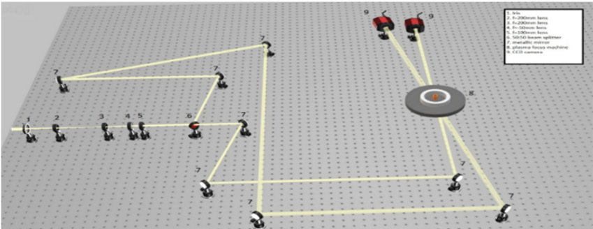
Figure 3. Schematic representation of the shadowgraphy setup
