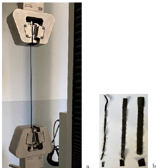
Figure 1. a) Velostat during the tensile test with PLA plates. b) Tears appeared after the test without PLA plates in 3 samples with different width.
