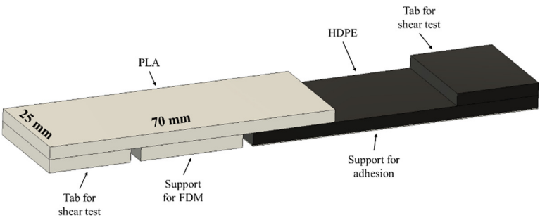
Figure 1. Final geometry of the test samples
