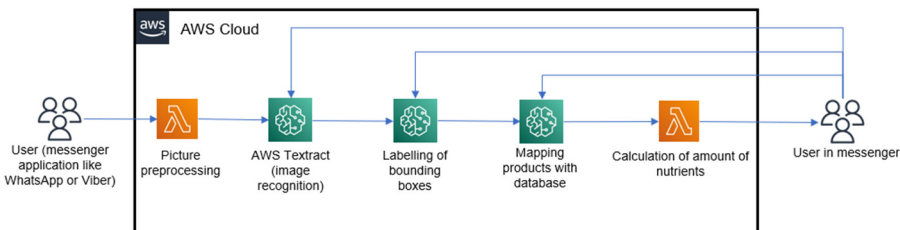
Figure 2. Chatbot architecture
