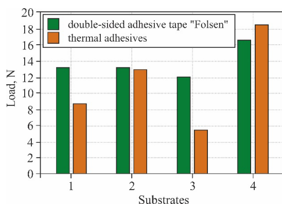
Fig. 16. Maximum load at which unsticking/tearing begins when the stretching speed is 1 mm min -1 (1 - paper “Rives traditional”, 2 - cardboard “Kreative Karton”, 3 - glossy laminate, 4 - matte laminate).
