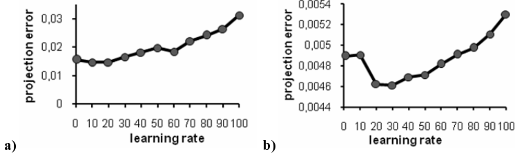
Fig 3. (a – Salinity dataset, b – Iris dataset) Dependence of the data projection accuracy on the learning rate \eta , \eta \in [1,100]
