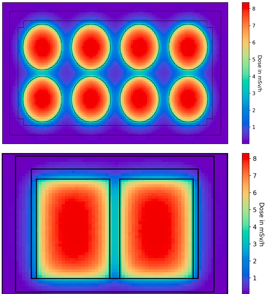
Fig. 9. Total effective dose rate (before decay, at time 0, Table 4) distribution top- and side-view for the waste container using G3-3 concrete.
