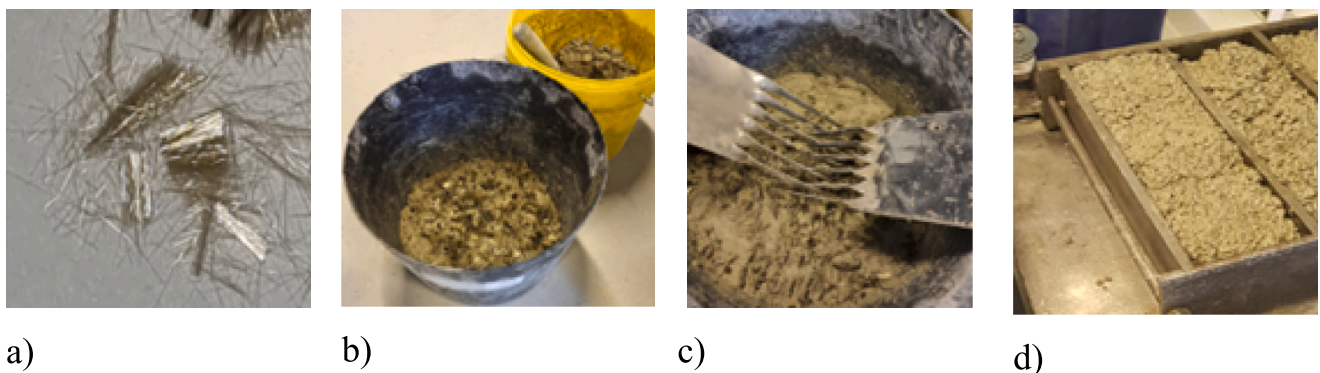
Fig. 2. A) BB short fibers; b) concrete layer with fibers on its surface; c) mixing; d) fresh fiber concrete cubes in moulds on the vibrating table.
