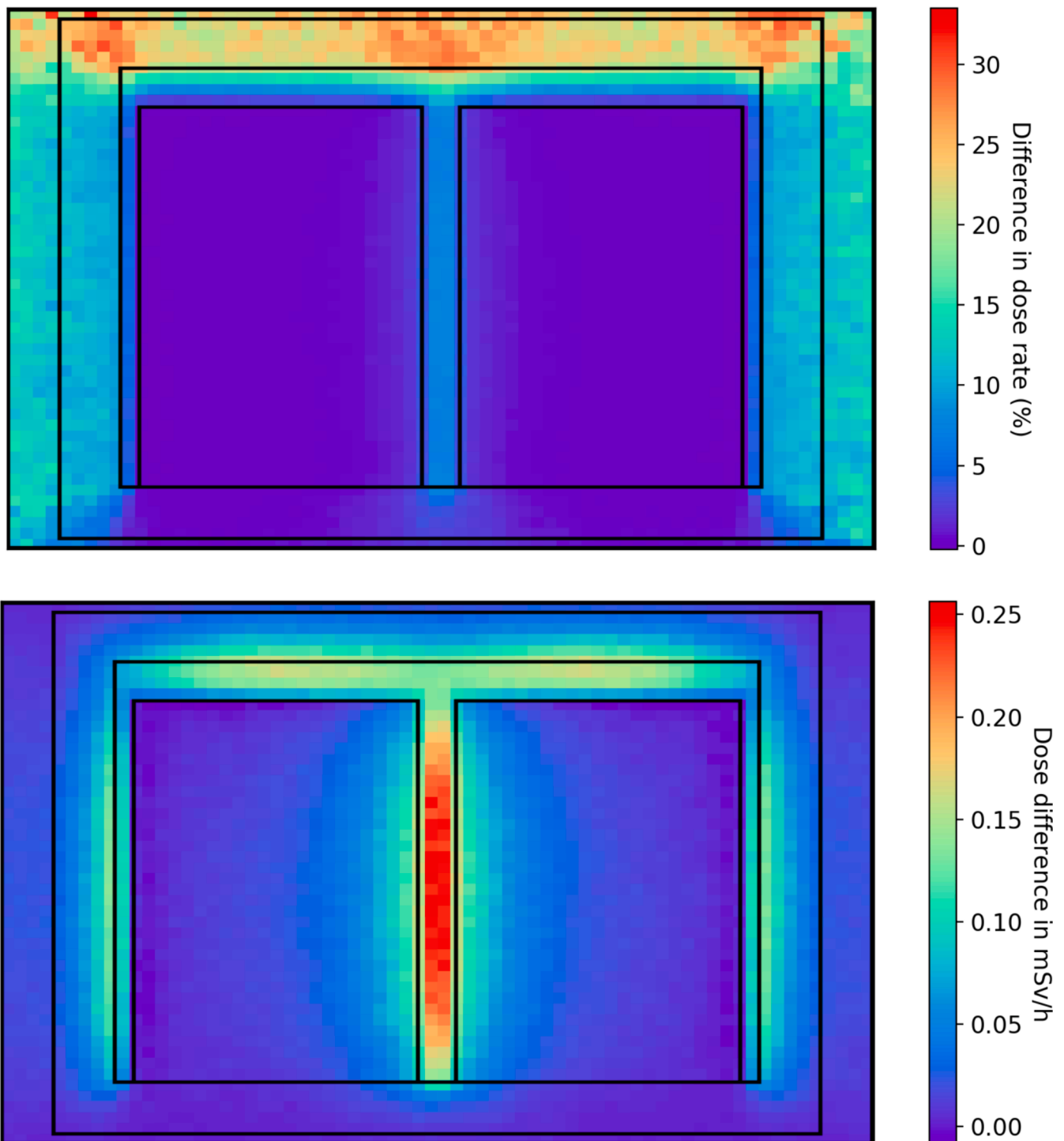
Fig. 10. Total effective dose rate (before decay, at time 0, Table 4) distribution difference in the waste container using cement paste and G3-3 concrete.
