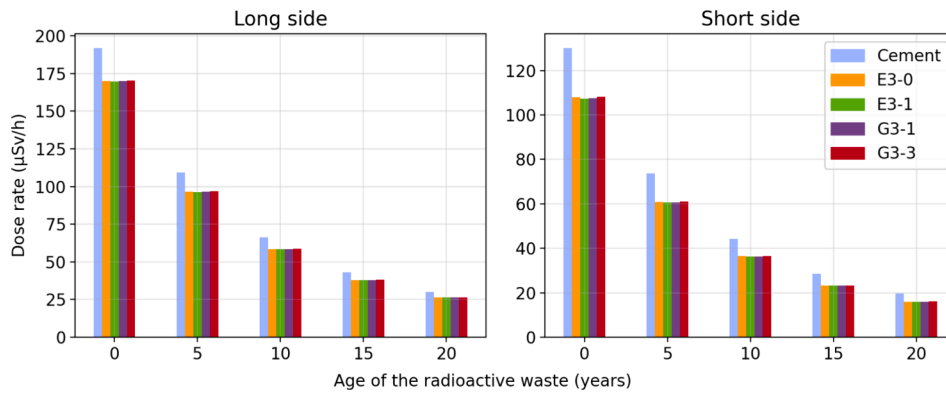
Fig. 8. Material-specific total averaged effective dose rates for both cell detectors in time.
