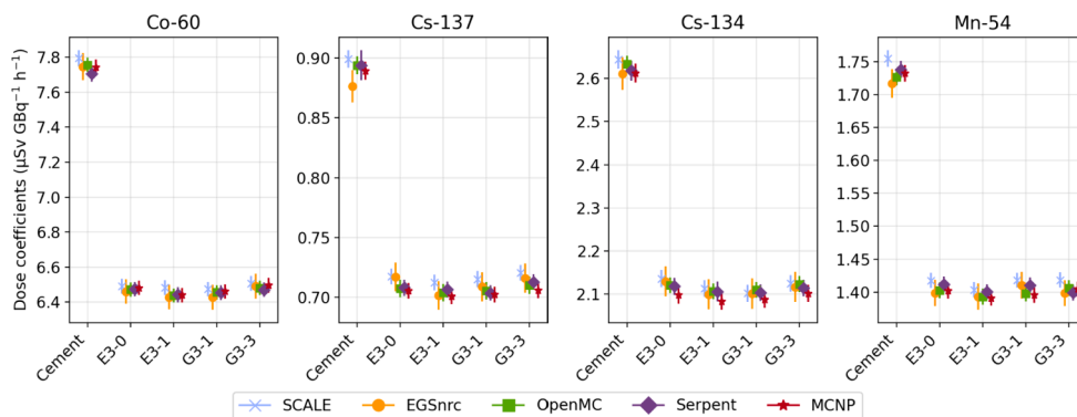
Fig. 5. Nuclide- and material-specific effective dose rate coefficient estimations for the detector at the short side of the container using SCALE, EGSnrc, OpenMC, Serpent, and MCNP.
