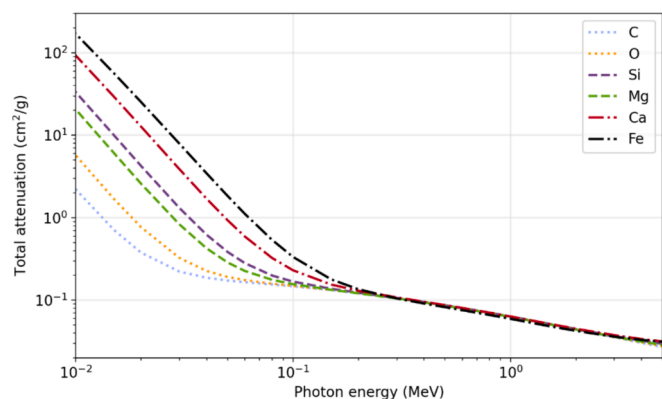
Fig. 6. Total attenuation factors describing the main elements of the additives. The attenuation factors were retrieved from NIST's XCOM database (Berger, et al., 2010).
