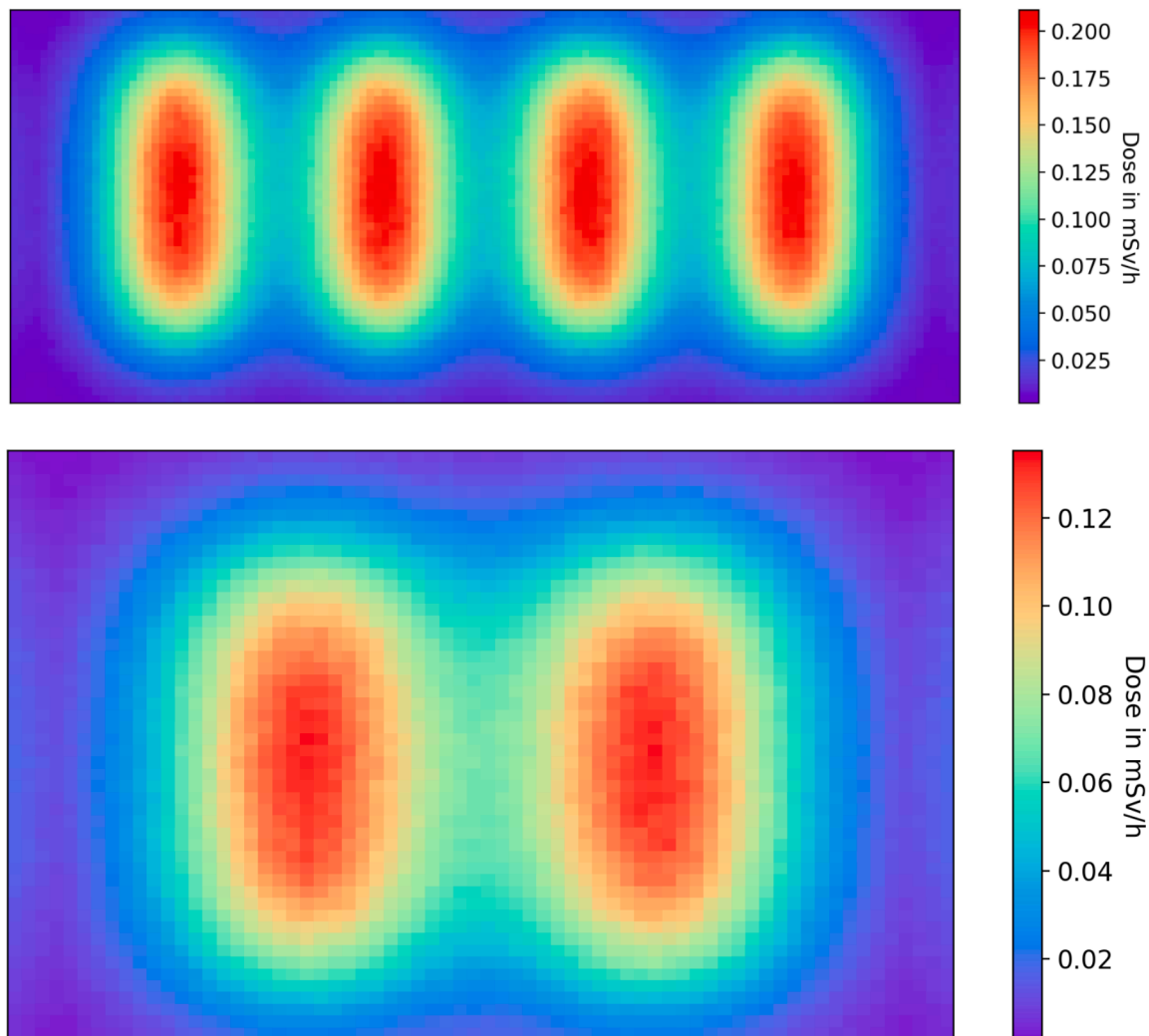
Fig. 11. Total effective dose rate distribution side-views (long side and short side) in the 10 cm layer of air around the container.
