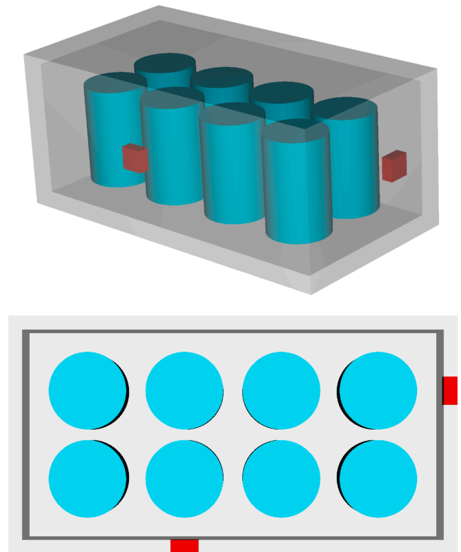
Fig. 3. Top and isometric view of detector locations for the Framatome-ANP waste package geometry visualized using EGSVIEW. Only the waste drums and surrounding air shown.
