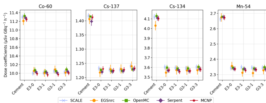
Fig. 4. Nuclide- and material-specific effective dose rate coefficient estimations for the detector at the long side of the container using SCALE, EGSnrc, OpenMC, Serpent, and MCNP.
