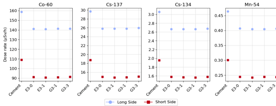
Fig. 7. Nuclide- and material-specific averaged effective dose rates (before decay, at time 0, Table 4) for both cell detectors.
