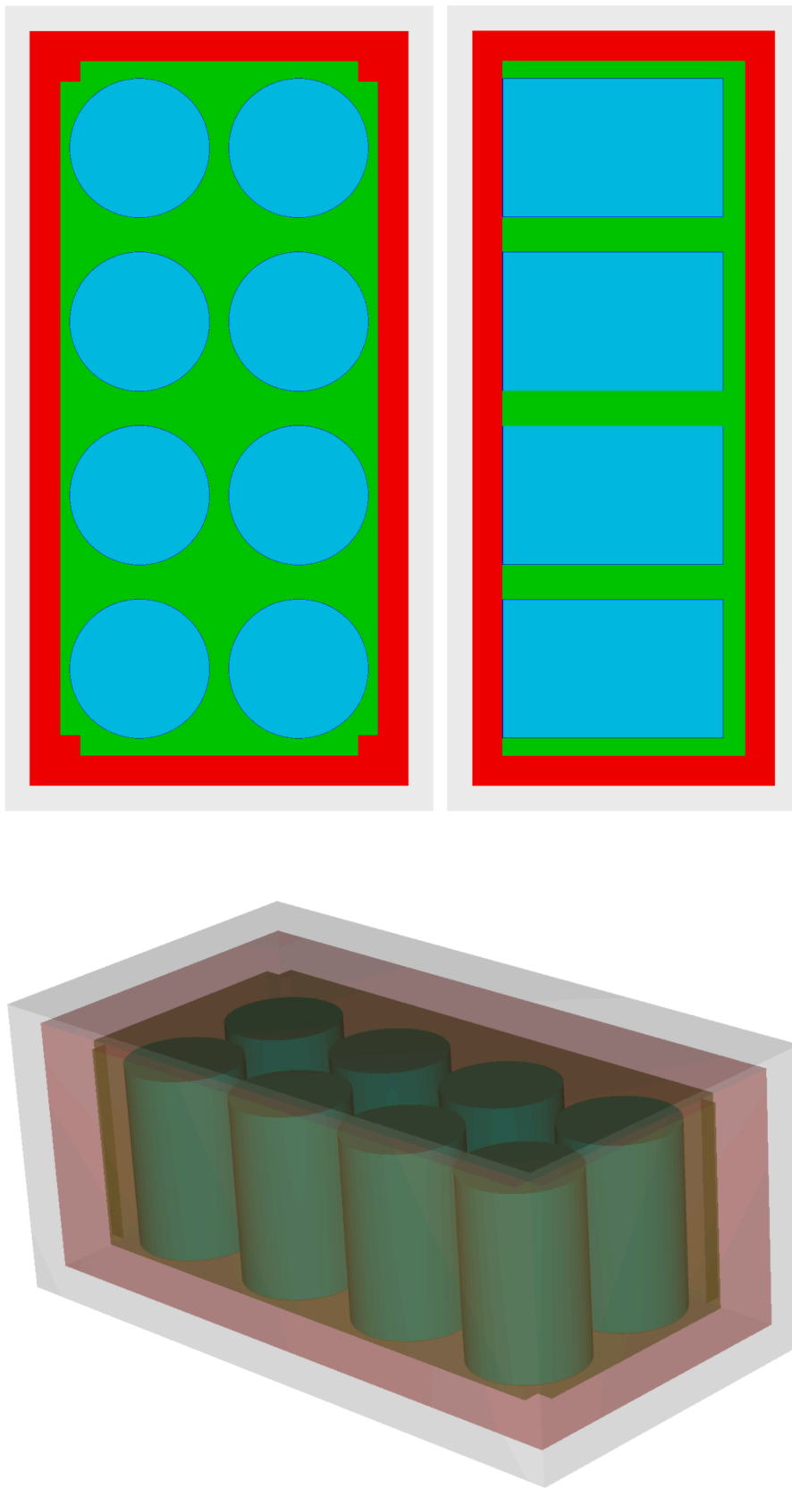
Fig. 1. Top-, side-, and isometric view of Framatome-ANP waste package geometry visualized using EGSVIEW.
