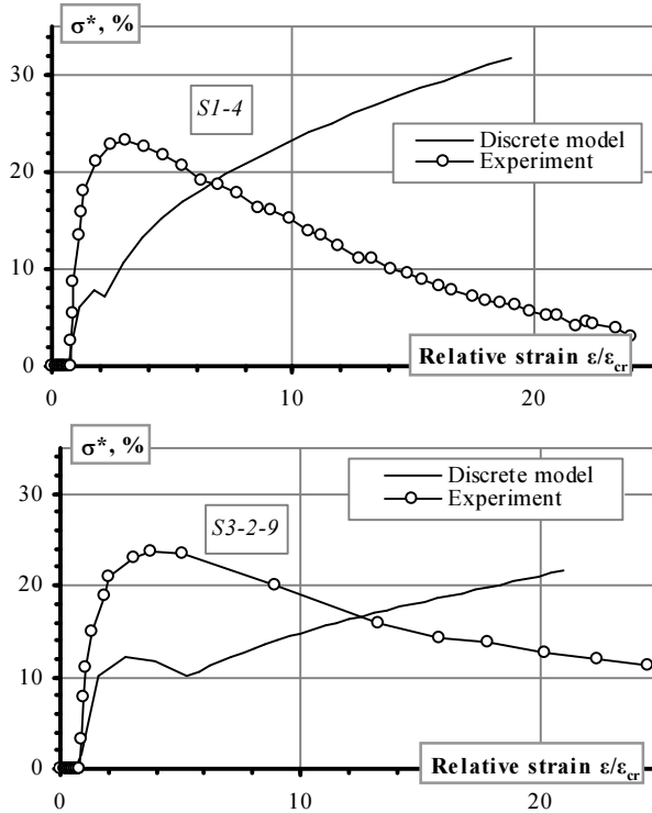
Fig. 7. Tension-stiffening diagrams of discrete model
