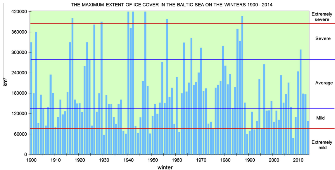
Fig. 14. Maximum annual ice extent in the Baltic Sea (prepared by Jouni Vainio, Finnish Ice Service).
