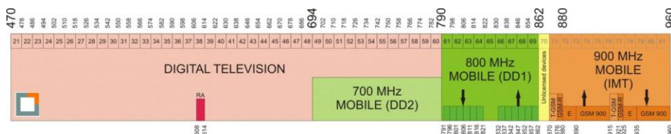
Fig. 1.5. Situation in 470–960 MHz frequency range
