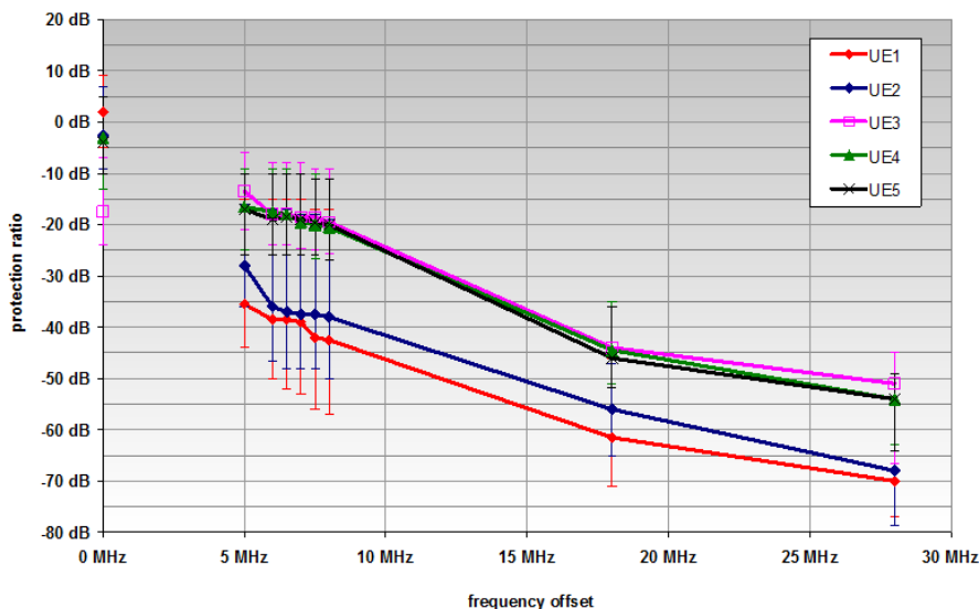
Fig. 3.12. Comparison of median protection ratio for all interfering signals at low level, Rx cat. 2 (Federal Network Agency 2013)
