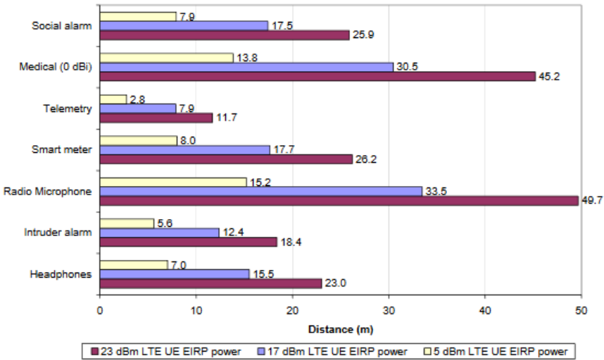
Fig. 3.13. Protection distances for simulated Long-Term Evolution with 50 RB: wanted level 10 dB above minimum sensitivity (ERA Technology 2011)
