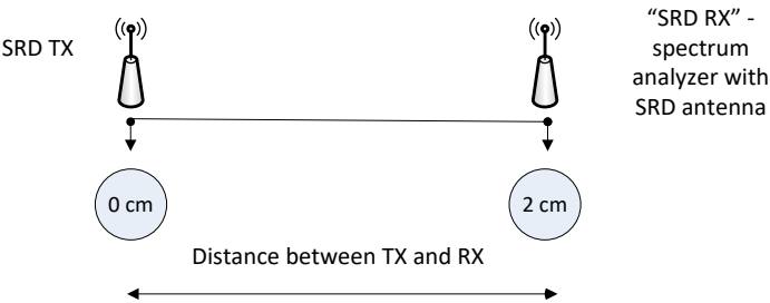
Fig. 3.1. Minimum Coupling Loss measurement situation
