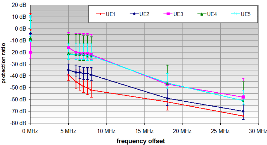
Fig. 3.11. Comparison of median protection ratios for all interfering signals at low level, Rx cat. 1 (Federal Network Agency 2013)
