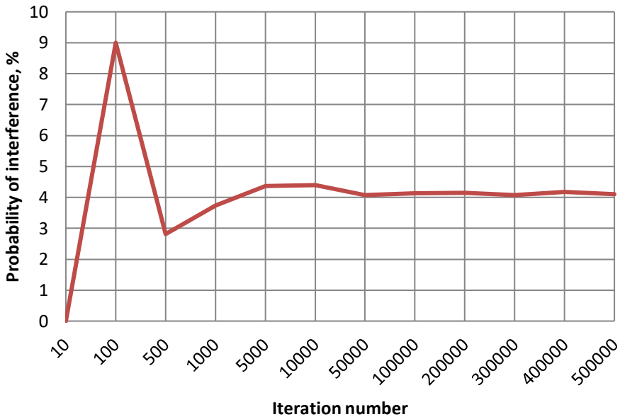
Fig. 2.6. Iteration number dependence on probability of interference
