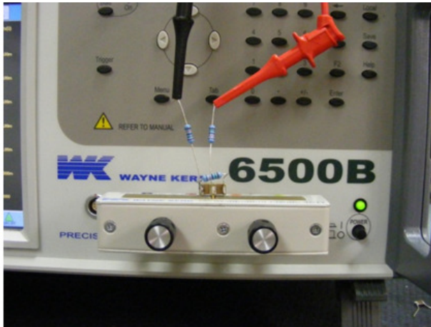
Fig. 4.2. Outside view of capacitor test setup
