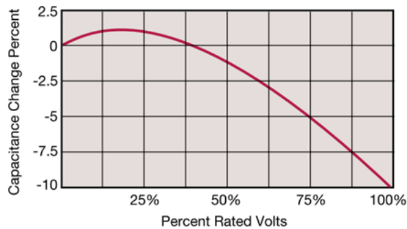
Fig. 1.20. Capacitance value change (in %) vs. DC voltage bias for AVX X7R capacitors (AVX, 2015)
