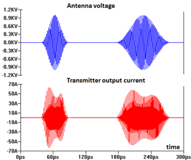
Fig. 1.6. NMR antenna voltage and the transmitter output current for 90 deg tipping (left) and 180 deg refocusing (right) pulses
