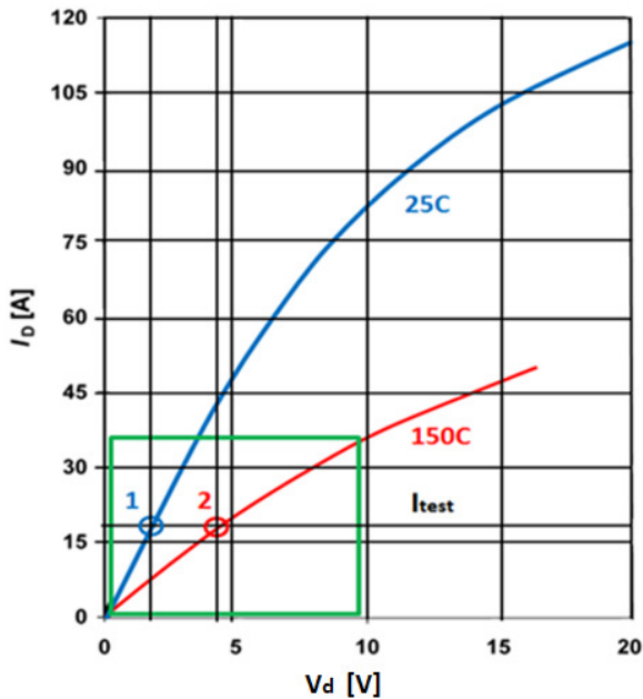
Fig. 1.19. I_d vs. V_d of MOSFET at 25^\circ C and 150^\circ C (IPB60R099, 2009)
