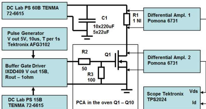
Fig. 3.2. Test setup for measuring the drain-to-source voltage drop vs. the drain current
