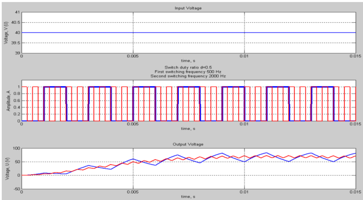
Figure 3.19. Execution of a boost converter with different switching frequency
