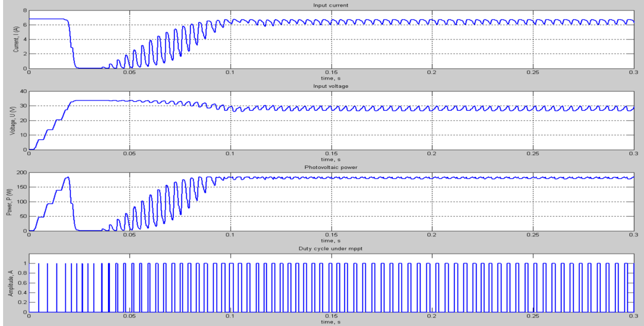
Figure 4.2. Current, voltage and power of photovoltaic module change in time after the implementation of MPPT algorithm
