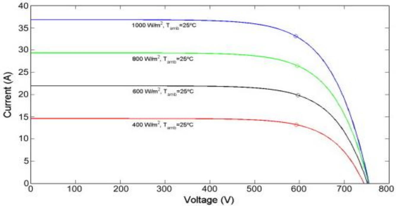
Figure 2.3. I-V curves on different solar irradiation [18]
