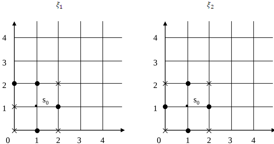
Figure 1. Two different TLC in second order neighbourhood scheme NN(2) with S^{(1)} and S^{(2)} points • and *, signed as respectively.
