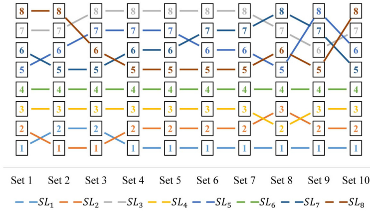
Fig. 4. Ranking variations of solutions across different weight sets.
