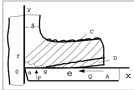
Figure 1. The process of the chip formation.
