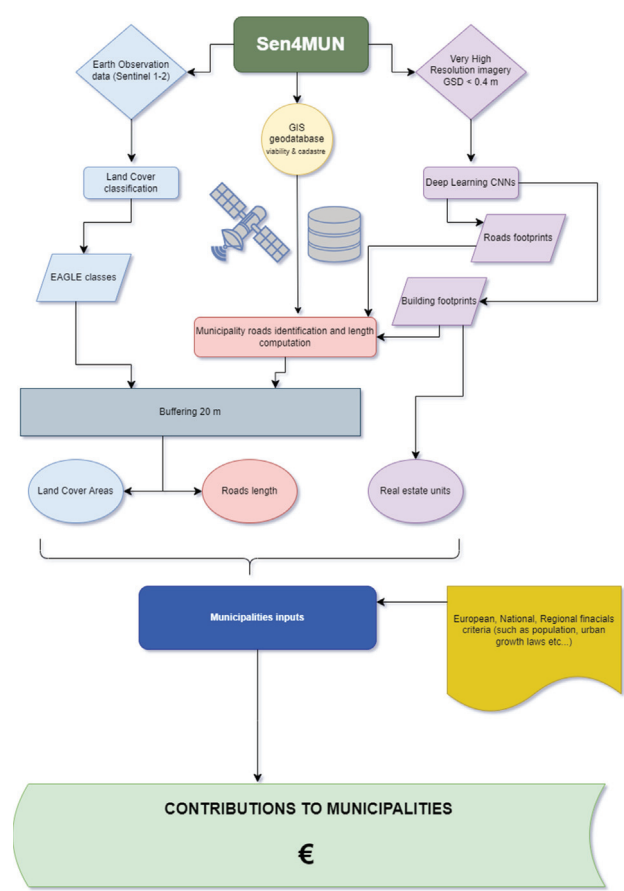
Figure 2. Sen4MUN workflow.
