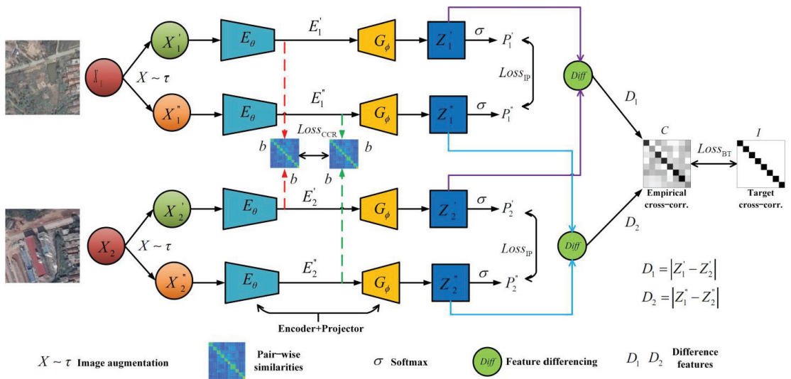
Figure 2. Flow chart of the BTCD algorithm.
