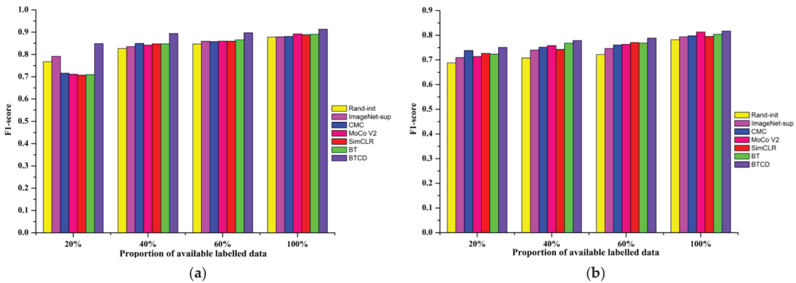
Figure 7. Performance (F1-score) of different pre-training methods evaluated using the improved UNet++ model under varying label availability. (a) LEVIR-CD. (b) SYSU-CD.
