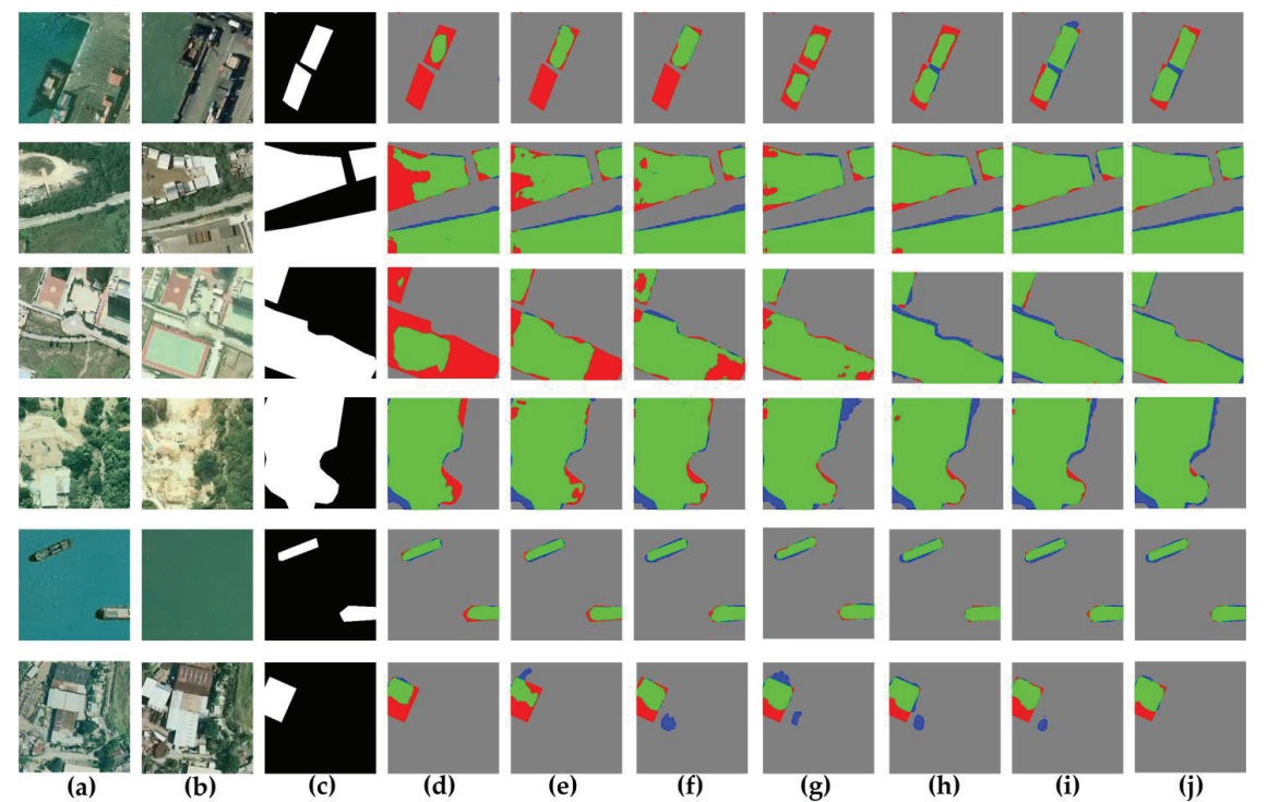
Figure 6. Visual comparisons of the UNet++ model applied to the SYSU-CD dataset using different pre-training methods. (a) Images at time T1, (b) Images at time T2; (c) ground truth; (d) Rand-init; (e) ImageNet-sup; (f) CMC; (g) SimCLR; (h) BT; (i) MoCo v2; and (j) BTCD. Gray: TN pixels; green: TP pixels; blue: FP pixels; red: FN pixels.
