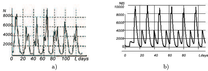
Figure 10. Modelling of Australian sheep-bowfly ( Lucilia cuprina ) population density. a) Nicholson's experimental data [24]. b) N(t) modelling results when \alpha = 10 ; \beta = 1 ; \gamma = 0.5 ; h = 4 ; n = 7.7 ; K = 2800 .
