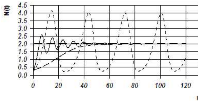
Figure 1. Solutions of equation (2.1): when h = 1 , r = 0.1 , K = 2 solution N(t) monotonically converges to K (dashed line); when h = 1 , r = 0.7 , K = 2 solution N(t) converges to K with oscillations near equilibrium (solid line); when h = 5.3 , r = 0.3 , K = 2 solution N(t) is periodic and stable (dotted line).
