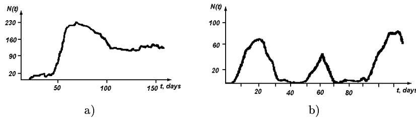
Figure 3. Daphnia density dynamics: a) T=18^{\circ}\text{C} , b) T=25^{\circ}\text{C} .
