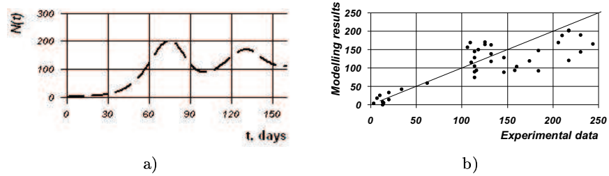
Figure 5. Modelling of Daphnia density dynamics when T=18^{\circ}\text{C} : a) simulation results when r = 0.1 , h = 12 and K = 135 , b) comparison of Pratt's [27] experimental data presented in Fig. 3a with modelling results. Correlation coefficient r = 0.83 .
