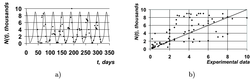
Figure 2. a) Comparison of Nicholson's [24] experimental data on laboratory population of Australian sheep-bowfly ( Lucilia cuprina ) with approximate solution N(t) (2.2), b) correlation coefficient r = 0.67 .
