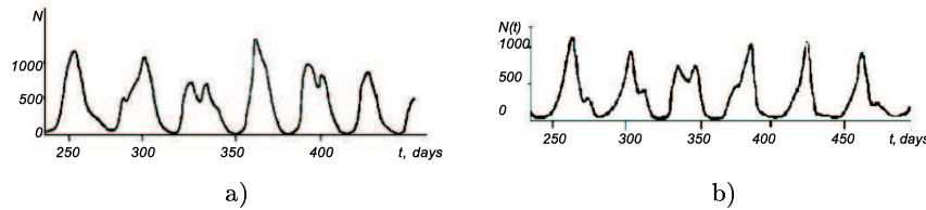
Figure 8. Adult flies' density dynamics when larva have got 25 g of meat per day. a) Nickolson's laboratory experiments data. b) Modelling results when T = 15 ; h_1 = 10 ; h_2 = 13 ; h_3 = 6 ; r_1 = 13.8 ; r_2 = 24 ; a = 0.495 ; b = 1.8 ; c = 0.715 ; \alpha = 3 ; K_1 = 350 ; K_2 = 700 .
