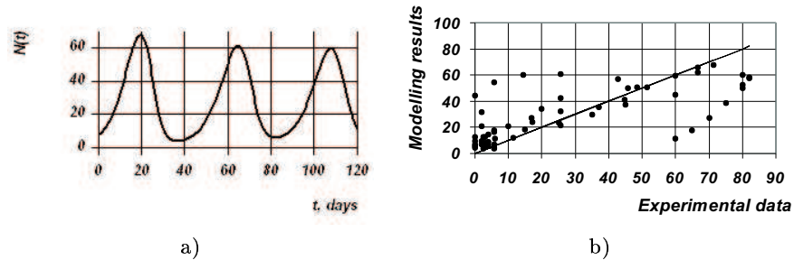
Figure 6. Modelling of Daphnia density dynamics when T=25^{\circ}\text{C} : a) simulation results when r = 0.18 , h = 9 and K = 30 . b) Comparison of Pratt's [27] experimental data presented in Fig. 3b with modelling results. Correlation coefficient r = 0.73 .
