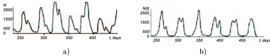
Figure 9. Adult flies' density dynamics when larva have got 50 g of meat per day. a) Nickolson's laboratory experiments data. b) Modelling results when T = 15 ; h_1 = 10 ; h_2 = 13 ; h_3 = 6 ; r_1 = 13.8 ; r_2 = 24 ; a = 0.495 ; b = 1.8 ; c = 0.715 ; \alpha = 3 ; K_1 = 900 ; K_2 = 1700 .
