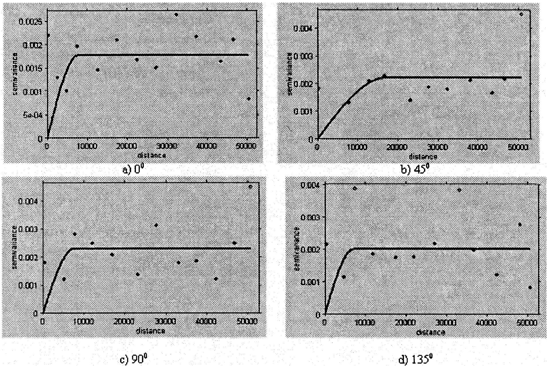
Fig. 4. Directional semivariogram.
