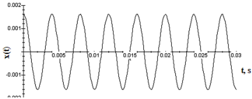
Fig. 4. The stable periodic solution of equation (33), when h_N = 0.001 s, \varepsilon = 0.3 .
