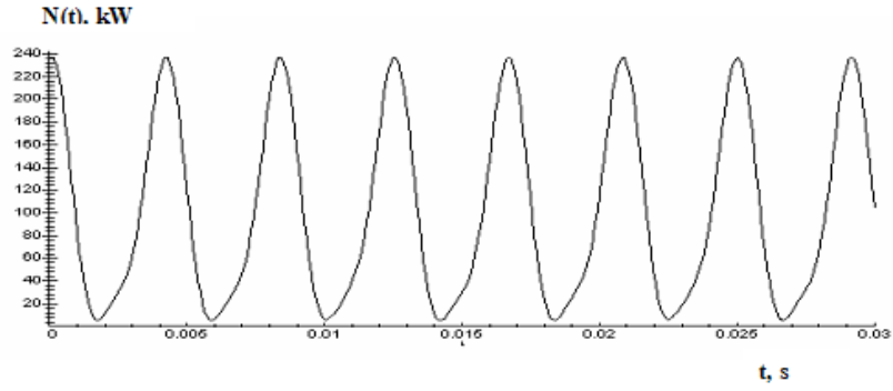
Fig. 2. The stable periodic solution of equation (3), when r_N = 1800 , N_0 = 100 kW.
