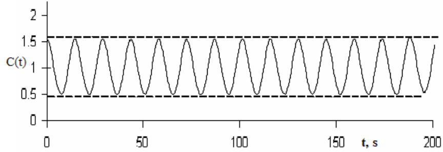
Fig. 3. The stable periodic solution of equation (4), when r_C = 0.1 , C_0 = 1 kW.
