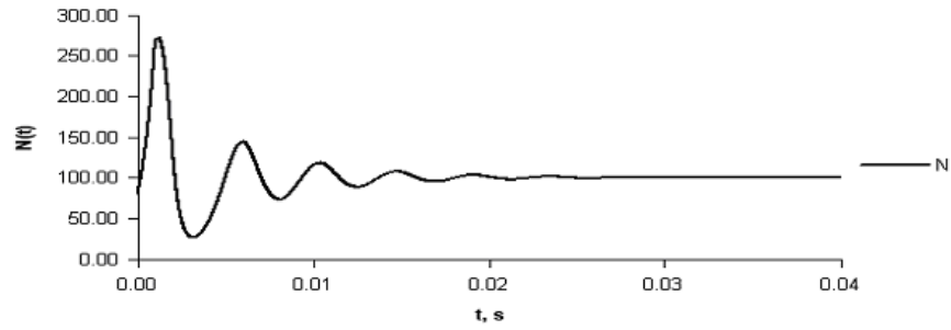
Fig. 5. The asymptotic stable solution of the differential equation (3), when h_N = 0.001 s, N_0 = 100 kW, r_N = 1.200 .
