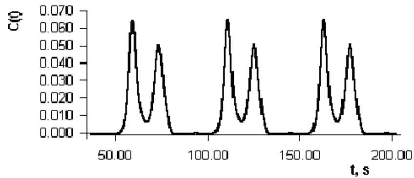
Fig. 12. The asymptotic stable solution of the differential equation (4), when N_0 = 5 kW, C_0 = 0.03 kW, r_C = 0.8 .
