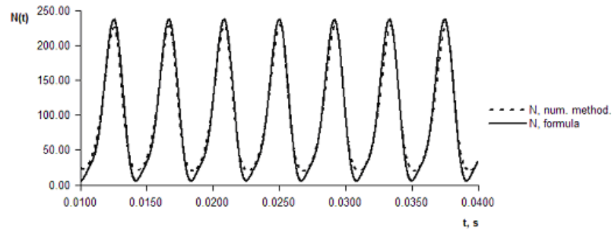
Fig. 9. The asymptotic stable solution of the differential equation (3), when h_N = 0.001 \text{ s} , N_0 = 100 \text{ kW} , r_N = 1800 .
