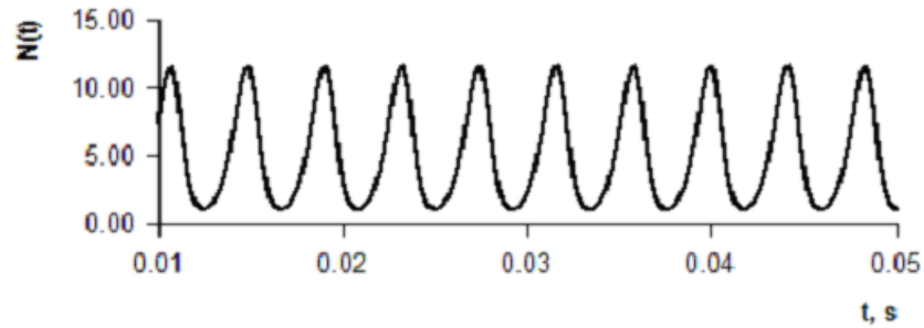
Fig. 11. The asymptotic stable solution of the differential equation (3), when h_N = 0.001 s, N_0 = 5 kW, r_N = 1800 .
