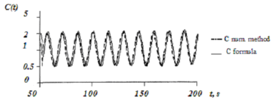
Fig. 10. The asymptotic stable solution of the differential equation (4), when N_0 = 100 \text{ kW} , C_0 = 1 \text{ kW} , r_C = 0.1 .
