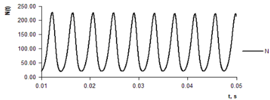
Fig. 7. The stable periodic solution of the differential equation (3), when h_N = 0.001 s, N_0 = 100 kW, r_N = 1800 .
