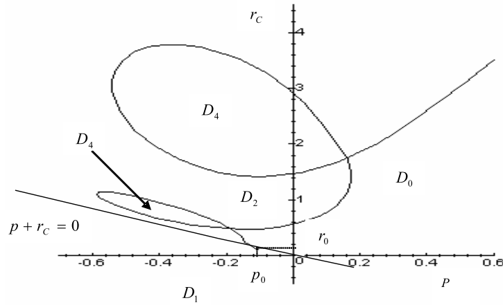
Fig. 1. The D -decomposition of quasi-polynomial (15).
