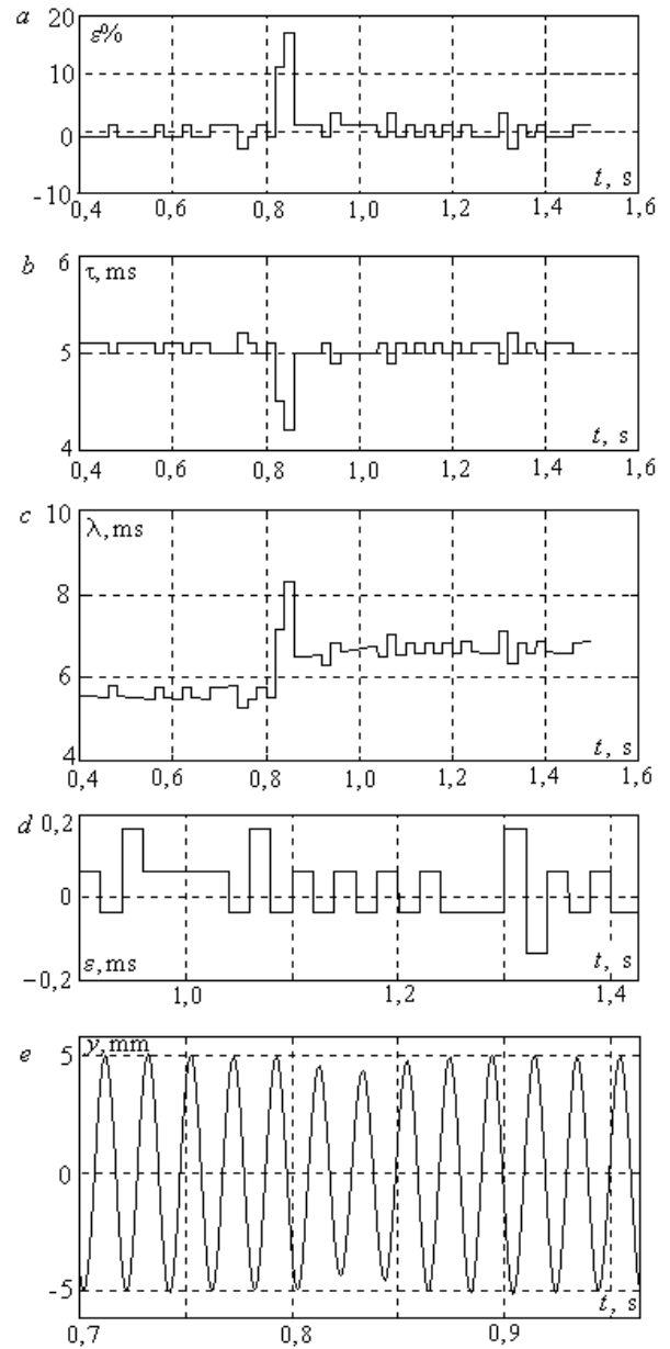
Fig. 5. Promoter's control process modeling results
