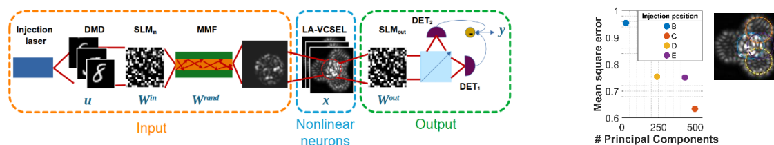
Figure 1. (a) Experimental setup of the ONN. (b) Computing power vs dimensionality represented by plotting MSE (mean square error) vs number of PCAs/ neurons in the LA-VCSEL.
