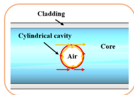
Figure 1. Schematic of the WGM resonator
