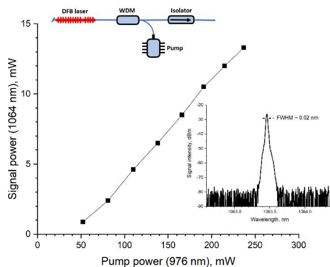
Figure 1. Dependence of output single-frequency signal power on pump power. Upper insert: scheme of DFB fiber laser; bottom insert: output spectrum of the DFM fiber laser.
