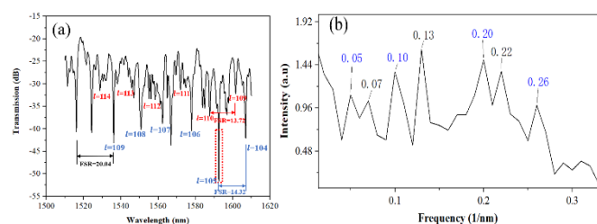
Figure 3. (a) The transmission spectrum of the optical fiber WGM cylindrical cavity resonator with diameter of 38 \mu\text{m} . (b) The corresponding spatial frequency spectrum.
