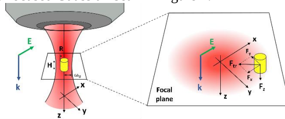
Figure 1. A cylindrical silicon nanoparticle placed in the focus of a linearly-polarized Gaussian beam. The inset shows the components of the optical force acting on the nanoparticle
