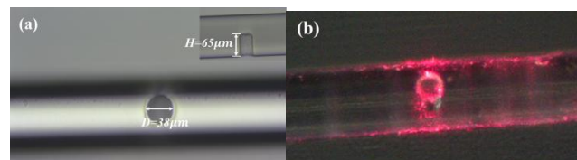
Figure 2. Microscope image of the WGM resonator. (a) Top view. Inset: the cross-section view. (b) Top view under the red light illumination.
