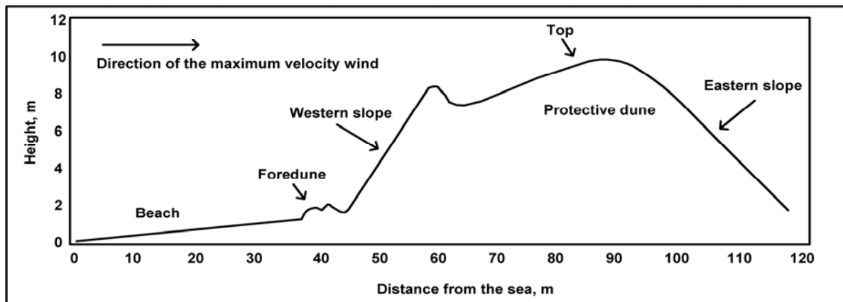
Fig 2. Ideal transverse profile of foredune and protective dune of the Curonian spit (Dubra, Grecevičius 2006)
