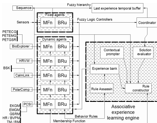
Fig. 3. The modified Fuzzy-Incremental Synchronous Learning Architecture of the Laboratory proposed by [1]
