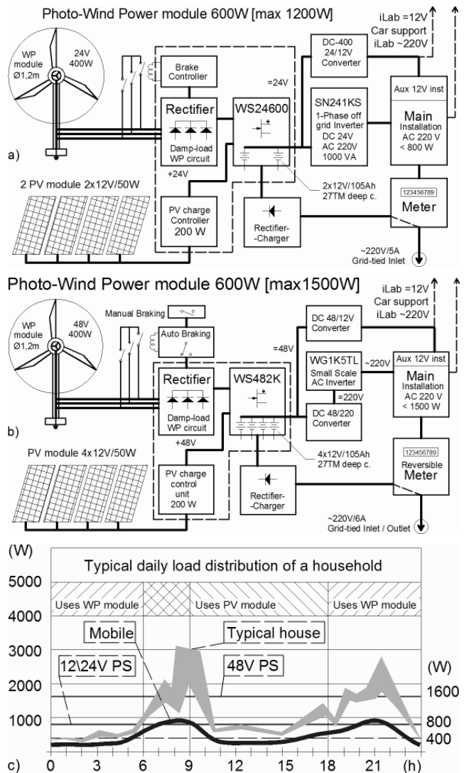
Fig. 2. The hybrid PV-WP supply system for mobile eco-social laboratory
