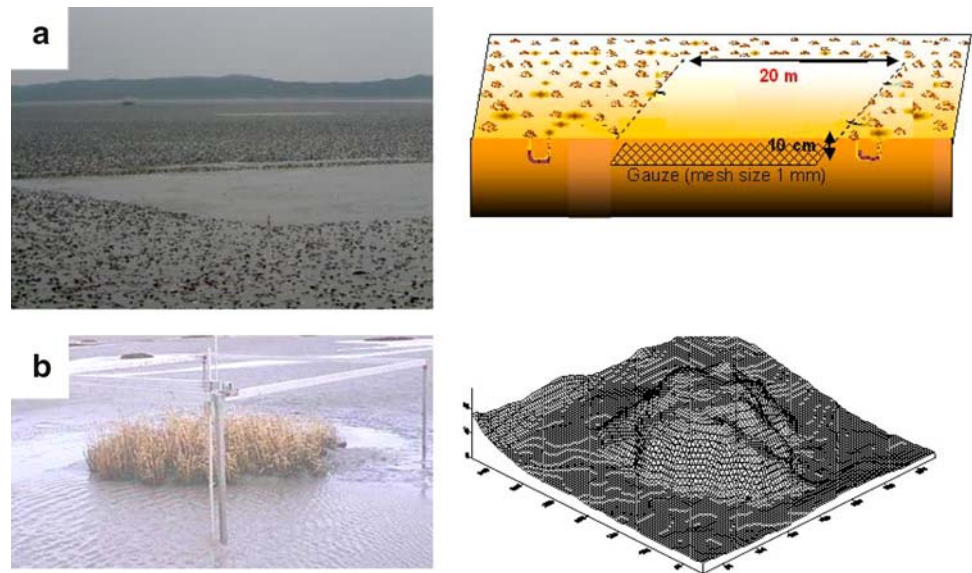
Fig. 1 Visual example of the major habitat modifying impact that can be exerted by a bioturbating endobenthic allogenic ecosystem engineer (a) and a sediment stabilising epibenthic autogenic ecosystem engineer (b). The smooth sediment surface on the mudflat was formed upon the exclusion of bioturbating lugworms ( Arenicola marina ) by burying a net in the sediment (a; picture courtesy of Nils Volkenborn). The presence of the cordgrass Spartina anglica causes the formation of a dome shaped tussock (b)
