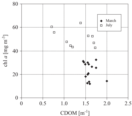
Figure 2. Chlorophyll a concentrations versus CDOM concentrations; the poor correlation ( r^2 = 0.37 ) is typical of case 2 waters
