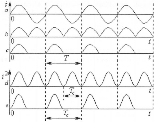
Fig. 1. Supply currents of oscillating motors
