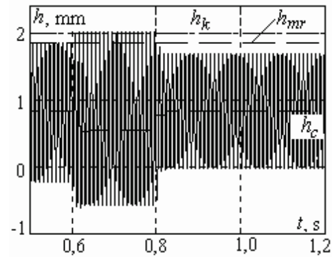
Fig. 6. Reaction of oscillations of uncontrolled drive to the sharp 25% decreasing and after 0,2 s sharp 50% increasing of the load when h_k=2,15 mm
