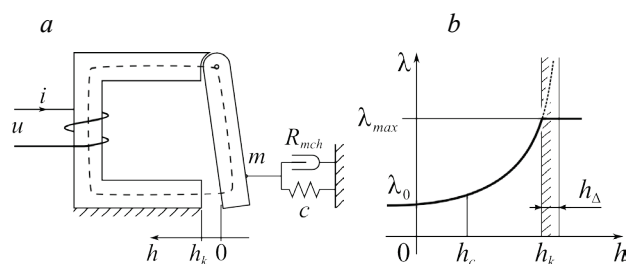
Fig. 1. Scheme of motor's construction and the load – a as well as the graph of permeance function – b
