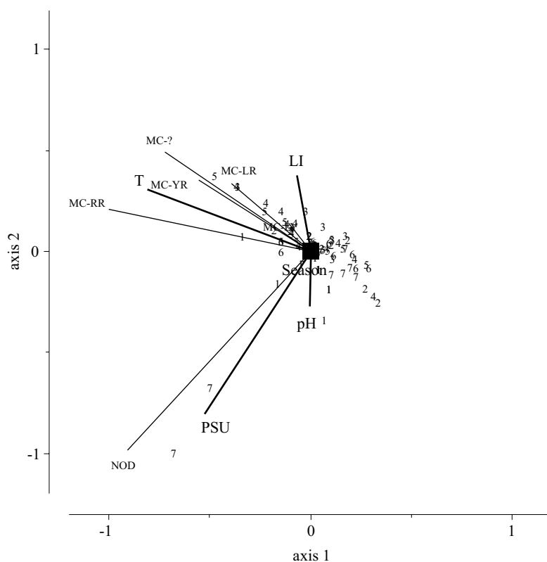
Figure 2. Biplot obtained by Redundancy Analysis. Light grey lines show response variables: MC-LR, MC-RR, MC-?, MC-YR, MC-LY, nodularin; bold lines indicate the explanatory variables: pH, salinity [PSU], temperature (T), light intensity (LI), season (summer, autumn); the numbers denote the stations
