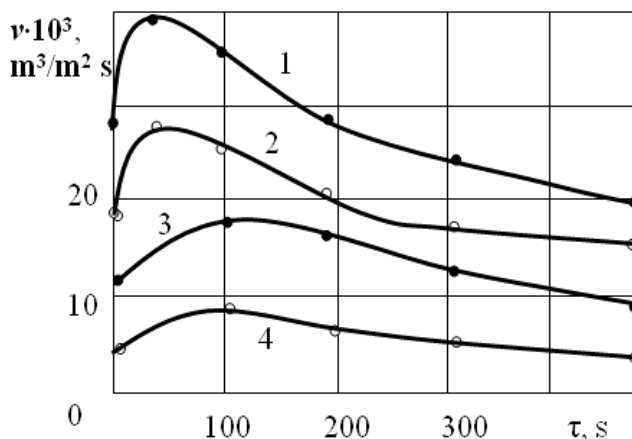
Fig. 7. Kinetics of the volumetric flow rate ( v ) of the styrene proceeding through the porous layer ( \Pi_0 = 0.39 ) of ceramics ( h = 10 mm) made from spherical particles \text{ZrO}_2/\text{CaO} . Faction 90...100 \mu\text{m} . Pressure differences (MPa): 1 – 0.05; 2 – 0.035; 3 – 0.025; 4 – 0.015
