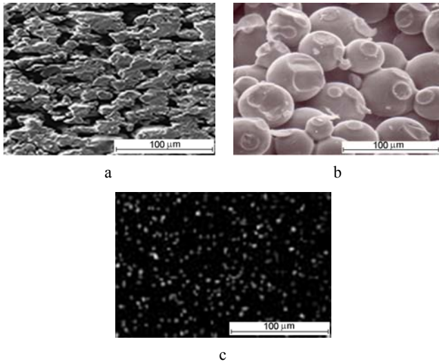
Fig. 1. The general view of the materials with developed porous structure: a – metal sample produced from plate form particles of reduced iron; b – the ceramic sample sintered from micro spheres \text{ZrO}_2/\text{CaO} ; c – the sample of the carbonaceous thermooxidized polyvinyl alcohol (PVA)
