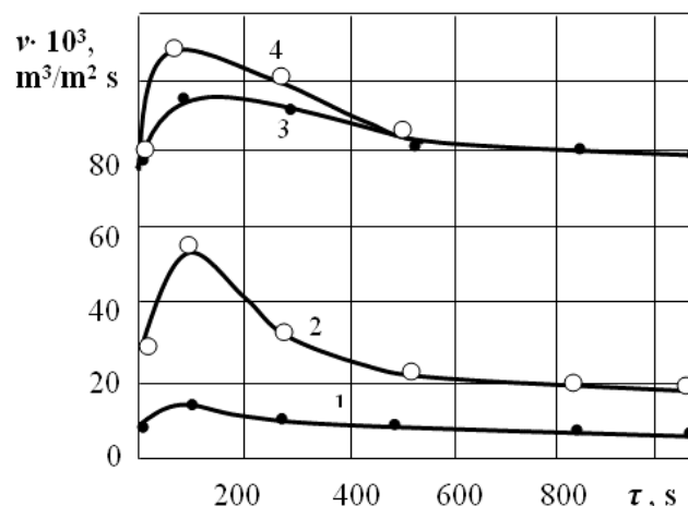
Fig. 5. Kinetics of the volumetric flow rate ( v ) of MMA-proceeding through porous layers (2 mm) from: 1 – ceramics \text{Al}_2\text{O}_3 ( I_0 = 0.19 , d_{II} = 28 \mu\text{m} ); 2 – porous alloy steel Cr-Ni-Ti ( I_0 = 0.19 , d_{II} = 28 \mu\text{m} ); 3 – carbonaceous PVA ( I_0 = 0.194 , d_{II} = 28 \mu\text{m} ) and 4 – carbonaceous PVA at presence 10 % LiCl ( I_0 = 0.195 , d_{II} = 32.3 \mu\text{m} )
