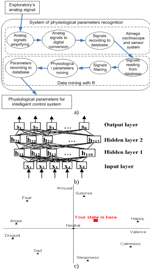
Fig. 2. Elements of physiological parameters recognition subsystem: a – concept models, b – multi-layer preceptron (MLP) to recognizing e-health aware state of an individual, c – emotional state allocation on continuous arousal-valence space
