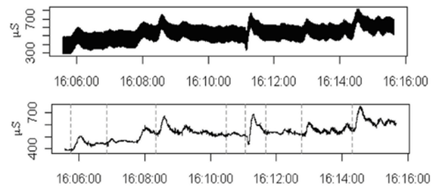
Fig. 3. SC signal filtering using Gaussian smoothing
