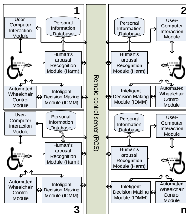
Fig. 1. The modified computer mediated communication model of the system by [5]
